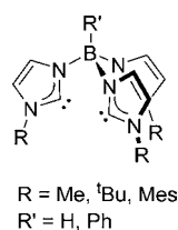
Figure 1. Tris(carbene)borate ligands based on imidazol-2-ylidene donors.
