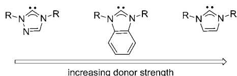
Figure 2. Relative donor strength of selected NHC ligands.
