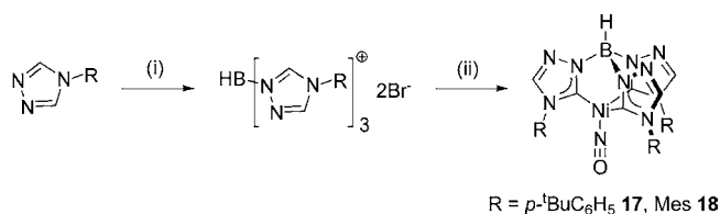
Scheme 4. Synthesis of HB(RTz) 3 NiNO Complexes 17 and 18 a
