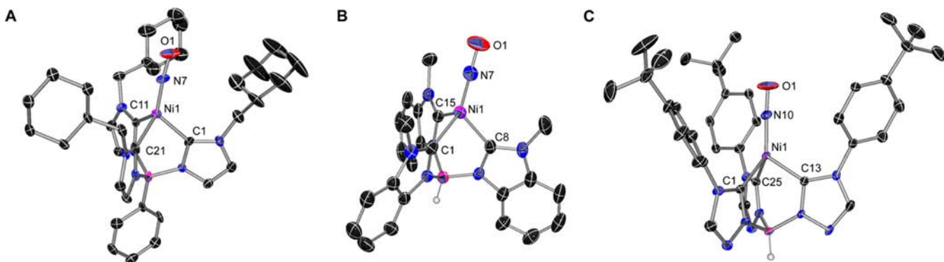
Figure 4. X-ray crystal structures of representative nickel nitrosyl complexes. Thermal ellipsoids shown at 50% probability, most hydrogen atoms omitted for clarity. (A) \text{PhB}(\text{CyCH}_2\text{Im})_3\text{NiNO} 14 . One of three independent molecules in the asymmetric unit. Selected bond lengths (Å) and angles (deg): Ni(1)–N(7) 1.643(10); Ni(1)–C(1) 1.982(11); Ni(1)–C(11) 1.939(11); Ni(1)–C(21) 1.974(13); N(7)–Ni(1)–C(1) 122.8(5); N(7)–Ni(1)–C(11) 123.2(5); N(7)–Ni(1)–C(21) 130.3(5); Ni(1)–N(7)–O(1) 173.7(11). (B) \text{HB}(\text{MeBz})_3\text{NiNO} 15 . One of four independent molecules in the asymmetric unit. Selected bond lengths (Å) and angles (deg): Ni(1)–N(7) 1.646(2); Ni(1)–C(15) 1.945(3); Ni(1)–C(1) 1.959(3); Ni(1)–C(8) 1.961(3); N(7)–Ni(1)–C(15) 118.85(11); N(7)–Ni(1)–C(1) 132.30(11); N(7)–Ni(1)–C(8) 123.90(11); O(1)–N(7)–Ni(1) 169.3(2). (C) \text{HB}(p\text{-}^t\text{BuPhTz})_3\text{NiNO} 17 . Selected bond lengths (Å) and angles (deg): Ni(1)–N(10) 1.640(2); Ni(1)–C(1) 1.979(3); Ni(1)–C(13) 1.989(3); Ni(1)–C(25) 1.985(3); N(10)–Ni(1)–C(1) 125.68(12); N(10)–Ni(1)–C(13) 122.51(12); N(10)–Ni(1)–C(25) 126.90(14); O(1)–N(10)–Ni(1) 176.3(3).
