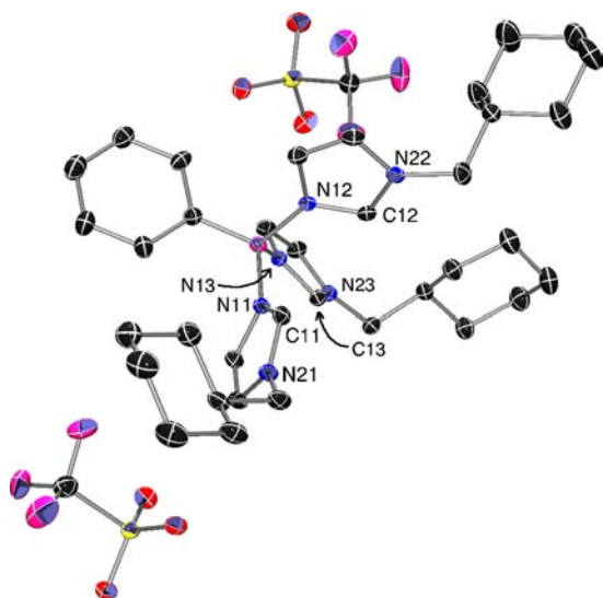
Figure 3. X-ray crystal structure of \text{PhB}(\text{CyCH}_2\text{ImH})_3\text{OTf}_2 6 . Thermal ellipsoids shown at 50% probability, hydrogen atoms omitted for clarity. Selected bond lengths (Å) and angles (deg): C(11)–N(11) 1.337(3); C(11)–N(21) 1.322(3); C(12)–N(12) 1.332(3); C(12)–N(22) 1.319(3); C(13)–N(13) 1.331(3); C(13)–N(23) 1.328(3); N(11)–C(11)–N(21) 109.8(2); N(12)–C(12)–N(22) 110.1(2); N(13)–C(13)–N(23) 110.2(2).
