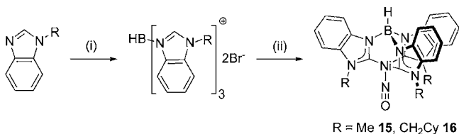
Scheme 3. Synthesis of HB(RBz) 3 NiNO Complexes 15 and 16 a
