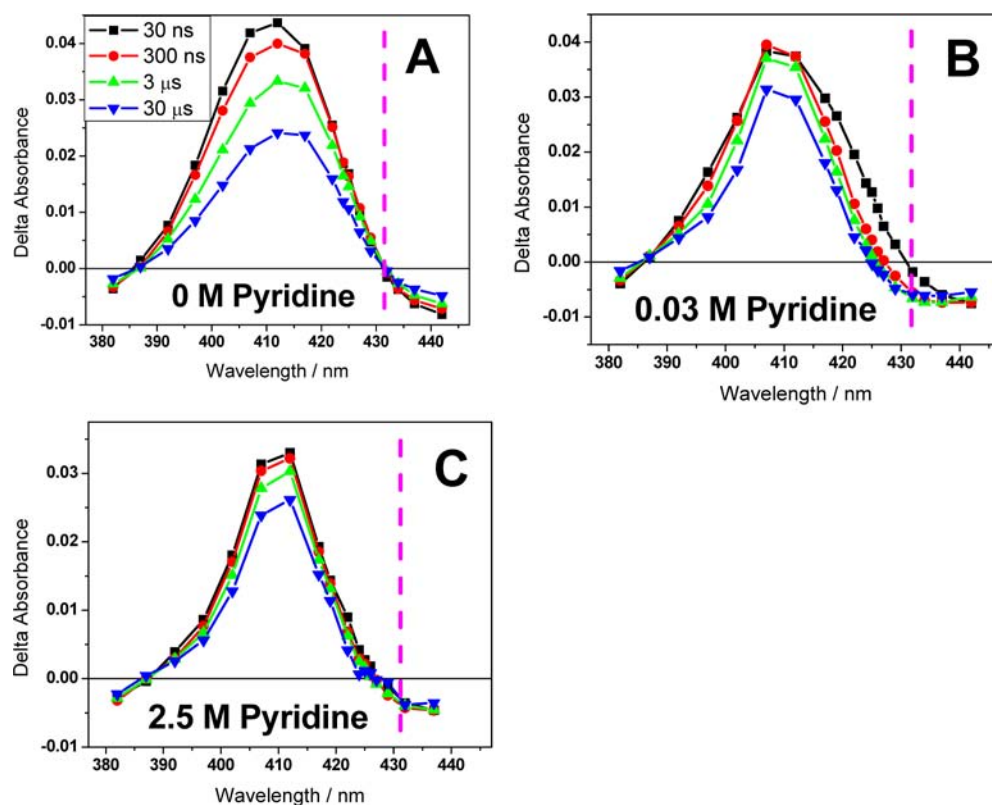
Figure 5. Transient absorption data collected at the indicated delay times following pulsed 532 nm laser excitation of a Co I P/TiO 2 thin film immersed in 0.1 M TBAClO 4 /CH 3 CN with the indicated pyridine concentrations. For reference, the vertical dashed line indicates the 432 nm isosbestic point for Co II to Co I reduction in the absence of pyridine.
