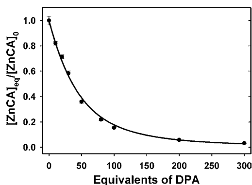
Figure 2. Inactivation of ZnCA after incubation with the \text{Zn}^{2+} chelator DPA. Fraction of active enzyme in each trial is calculated using the rate of ZnCA-catalyzed hydrolysis of p -nitrophenyl acetate ( p -NPA) in various concentrations of DPA. Catalytic rate of each trial then was normalized with the uninhibited hydrolysis (i.e., the same as [\text{ZnCA}]_0 with 0 equiv of DPA). All values reported are averages of at minimum 3 trials, and error values are derived from standard deviation. Reactivity was monitored by measuring formation of p -nitrophenol ( \epsilon_{404} = 17\,300 \text{ M}^{-1}\text{cm}^{-1} ). All trials done in the presence of dipicolinic acid (DPA) were completed after a 24 h incubation period at room temperature to ensure all solutions achieved equilibrium. Regression line is derived from eq 9.
