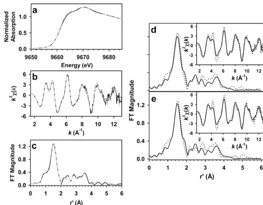
Figure 6. (left) Comparisons of the XAS data obtained for as-isolated (solid black line) and reconstituted (dashed gray line) ZnCA. XANES spectra (a), k^3\chi(k) EXAFS spectra (b), and Fourier transforms (c, k = 1.5\text{--}13.0 \text{ \AA}^{-1} ) are essentially superimposable. Fourier transforms of the unfiltered k^3\chi(k) EXAFS data (insets) of as-isolated CA (d) and reconstituted CA (e). Experimental data are represented by dotted lines, while best fits (given in bold in Table 2) are shown as solid black lines.
