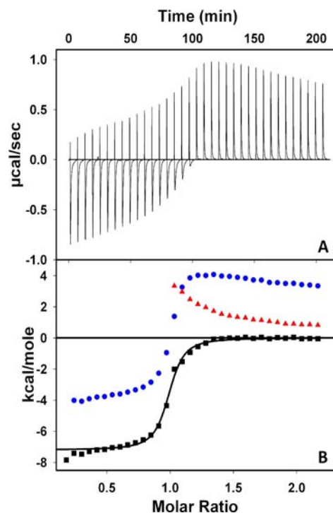
Figure 4. Isothermal titration calorimetry data of zinc binding to apoCA. (A) Raw data from titration of a 1.5 mL cell containing 80 \mu\text{M} apoCA was titrated with 35 \times 3 \mu\text{L} of 2.26 mM Zn(\text{NO}_3)_2 in 100 mM PIPES at pH 7.4. (B) Blue: Integrated raw data. Red: Integrated Zn^{2+} -buffer background titration. Black: Corrected Zn^{2+} binding isotherm and the best associated fit for a one-site binding model. Average thermodynamic parameters associated with Zn^{2+} binding to apoCA are reported in Table 1.
