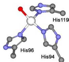
Figure 1. Zinc coordination site structure of human carbonic anhydrase II. Image generated using Accelrys Discovery Studio Visualizer 2.5 from coordinates associate with 2CBA.
