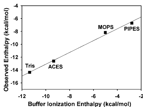
Figure 5. Plot of the addition of observed enthalpy from ITC and metal–buffer interaction enthalpy ( \Delta H_{\text{ITC}} + \Delta H_{\text{Zn-Buffer}} ) versus buffer ionization enthalpies ( \Delta H_{\text{H-Buffer}} ) in various buffers at pH 7.4. Values for \Delta H_{\text{ITC}} , \Delta H_{\text{Zn-Buffer}} , and \Delta H_{\text{H-Buffer}} in various buffers are listed in Tables 1 and S1. Linear regression values: y = 0.92x - 3.92 . R^2 = 0.99 .
