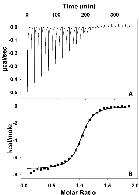
Figure 3. Isothermal titration calorimetry data of zinc binding to apoCA. (A) Raw data from titration of a 1.5 mL cell containing 60 \mu\text{M} apoCA was titrated with 30 \times 3 \mu\text{L} of 1.73 mM Zn(\text{NO}_3)_2 in 100 mM ACES at pH 7.4. Injection interval is 12 min. (B) Integrated isotherm and best associated fit for a one-site binding model. Average thermodynamic parameters associated with Zn^{2+} binding to apoCA are reported in Table 1.
