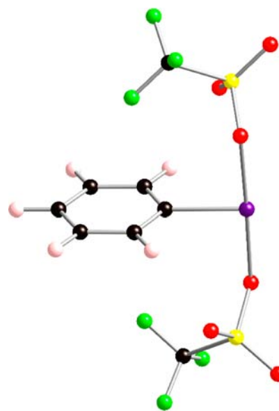
Figure 4. Optimized geometry of PhI(OTf) 2 .
