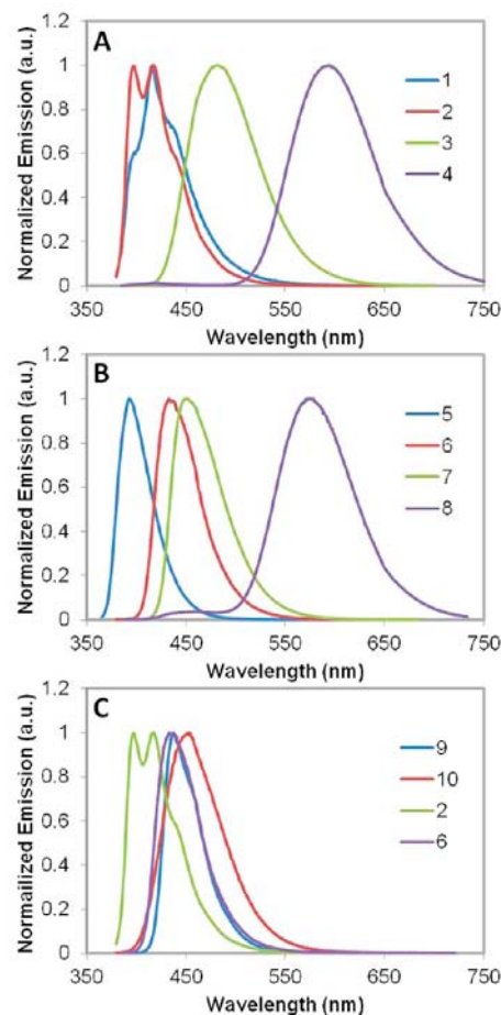
Figure 2. Photographs and steady-state emission spectra of \text{BF}_2\text{bdk} s 1–10 in \text{CH}_2\text{Cl}_2 ( \lambda_{\text{ex}} = 369\text{ nm} ).
