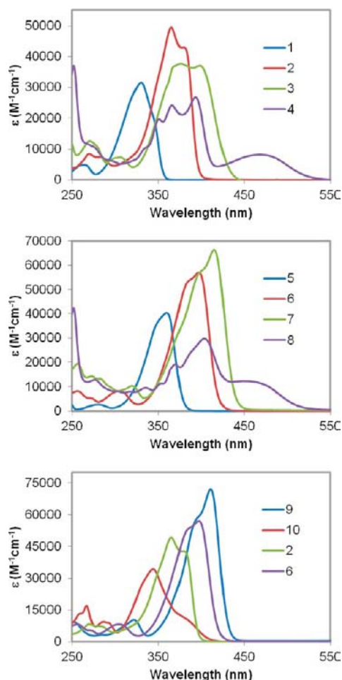
Figure 1. Absorption spectra of \text{BF}_2\text{bdk} complexes 1–10 in \text{CH}_2\text{Cl}_2 .
