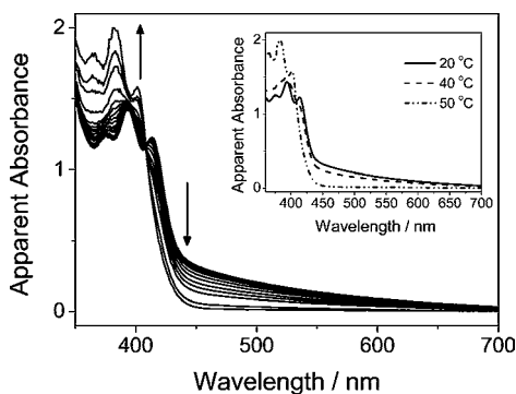
Figure 8. UV–Vis absorption spectral traces of the sol–gel phase transition of complex 4 in hexane upon an increase in the temperature from 10 to 50 ^{\circ}\text{C} . Inset: spectral traces at 20, 40, and 50 ^{\circ}\text{C} .
