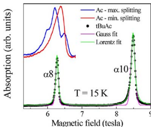
Figure 12. A comparison between the hard-plane HFEPR spectra for 1 and 3·MeOH at 15 K and 51.5 GHz. Data for 1 , which have been offset for clarity, are only available below 6.8 T. The solvent disorder in 1 gives rise to fine structures (high- and low-field shoulders) that are well resolved from the central peak for some field orientations within the hard plane (blue curve), and unresolved for others (red curve). 37d These fine structures are completely absent in the data for 3·MeOH. The thin green and magenta curves are Lorentzian and Gaussian fits to the data, respectively.
