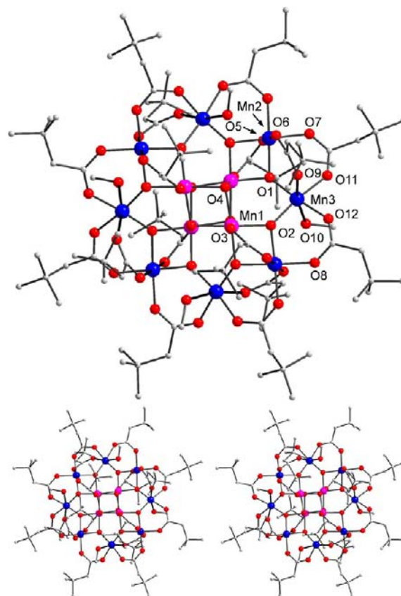
Figure 1. PovRay representations of partially labeled 3 and MeOH solvent molecule (top), and a stereoview (bottom). Color code: Mn IV purple; Mn III blue; O red; C gray.
