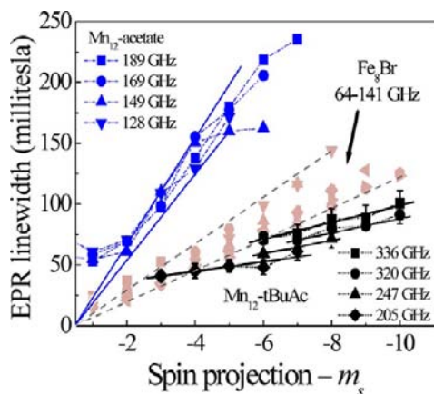
Figure 11. The full-width-at-half-maximum (fwhm) deduced from Gaussian fits to easy-axis HFEPR data obtained for three different S = 10 SMMs for a range of frequencies: 1 at 20 K (blue data); 37c \text{Fe}_8\text{Br} at 10 K (light gray data); 37c and \text{Mn}_{12} -tBuAc (3·MeOH) at 25 K (black data). The horizontal axis denotes the m_s value for the level from which the EPR transition was excited. See main text and eq 12 for explanation of the data.
