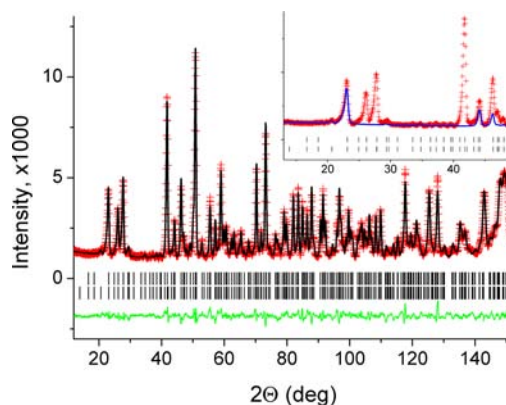
Figure 7. Rietveld plot for the \text{Na}_2\text{CoP}_2\text{O}_7 NPD data at 3 K. The red crosses, black solid lines, and green solid lines indicate the observed and calculated curves and their difference, respectively. The two rows of black tick marks indicate position of the nuclear (top) and magnetic (bottom) diffraction peaks. The blue curve in the inset shows magnetic contribution. R_p = 4.29\% , R_{wp} = 5.46\% , R_{Bragg} = 4.36\% , \chi^2 = 6.01 , R_{mag} = 6.69\% .
