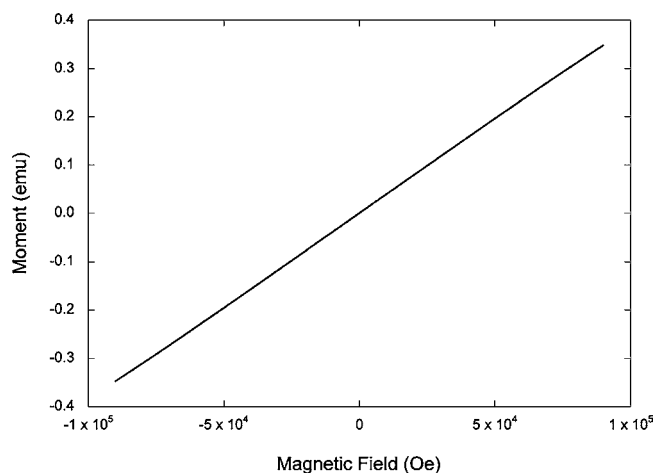
Figure 4. Magnetization as a function of field for Na 2 CoP 2 O 7 measured at 2 K.
