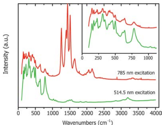
Figure 3. Vibrational Raman and electronic fluorescence spectra collected at ambient conditions for \text{CaZrTi}_2\text{O}_7 zirconolite samples using 785 and 514 nm laser excitation. The strong peaks observed above 1000\text{ cm}^{-1} with the red laser line are due to electronic transitions of a rare earth cation (likely \text{Nd}^{3+} ) present as a trace impurity within the sample. The inset shows the vibrational Raman spectra obtained with both laser excitations.
