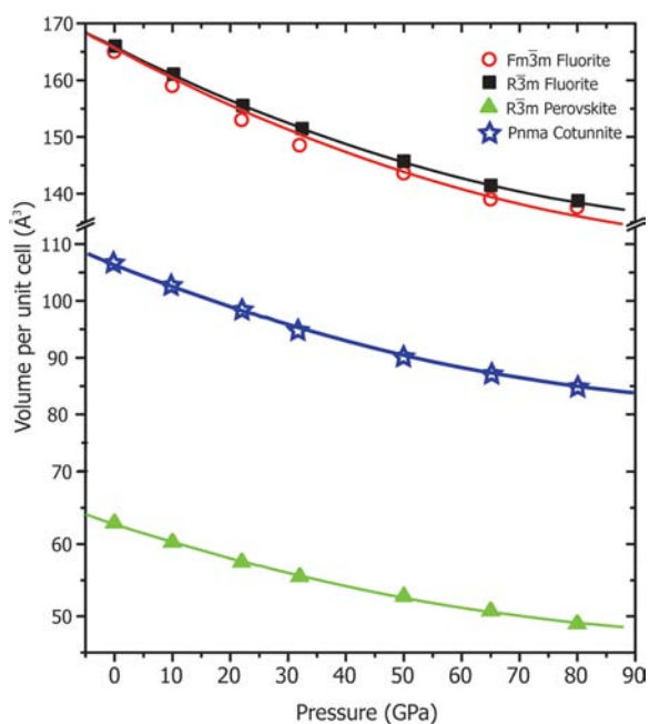
Figure 13. V(P) relations for the decompression of the high pressure phase of CaZrTi_2O_7 (zirconolite-III) analyzed using four different structural models. The bulk modulus values for the four models are as follows: (1) Fm\bar{3}m fluorite: K_0 = 225(19) GPa, K_0' = 6.8(0.9) . (2) R\bar{3}m fluorite: K_0 = 282(12) GPa, K_0' = 4.7(0.2) . (3) R\bar{3}m perovskites: K_0 = 208(12) GPa, K_0' = 3.5(0.2) . (4) Pnma cotunnite: K_0 = 239(19) GPa, K_0' = 5.1(0.6) .
