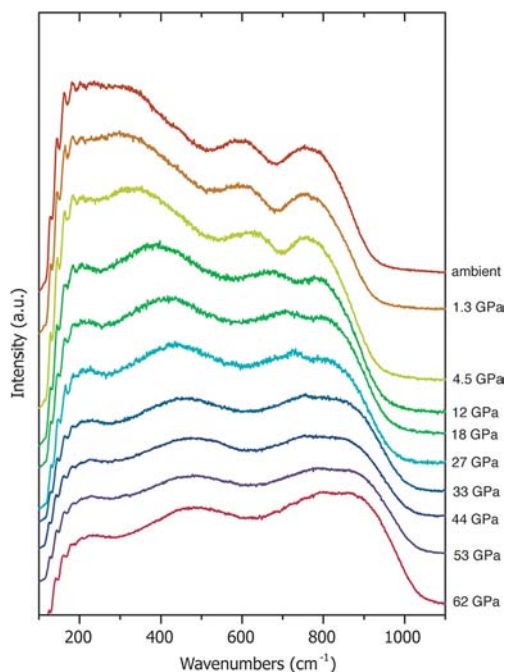
Figure 5. Raman spectra of zirconolite during decompression at ambient temperature in N_2 pressure transmitting medium obtained using 514.5 nm laser radiation.
