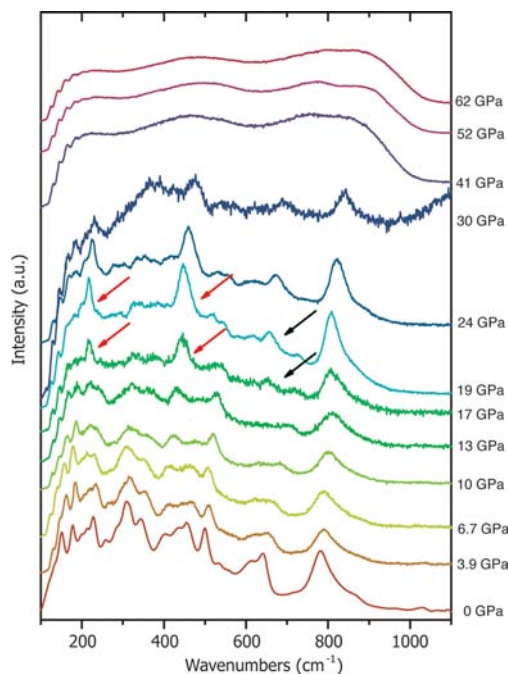
Figure 4. Raman spectra of zirconolite during compression at ambient temperature in \text{N}_2 pressure transmitting medium obtained using 514.5 nm laser radiation. The full spectral compression data up to a final pressure of 62 GPa are shown with selected patterns highlighting the appearance of new Raman peaks associated with the onset of a phase transition.
