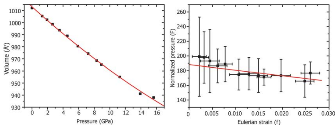
Figure 7. (left) V(P) plot for the C2/c phase of \text{CaZrTi}_2\text{O}_7 up to P \sim 15 GPa. Data were fitted using a third order Birch–Murnaghan equation of state. (right) The compressibility is further refined using a reduced variable normalized pressure ( F ) vs Eulerian strain ( f ) providing compressibility values of K_0 = 188(15) GPa; K_0' = 3.6(1) .
