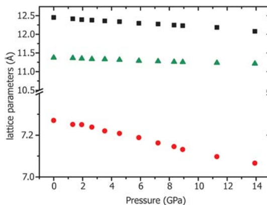
Figure 6. Plot of the lattice parameters of CaZrTi_2O_7 ( C2/c ) as a function of pressure up to 14 GPa. The black squares, red circles, and green triangles are representative of the a , b , and c lattice parameters, respectively. The values have been determined using Le Bail refinement.
