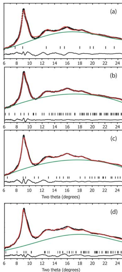
Figure 12. Structural refinement of the recovered zirconolite sample at ambient conditions following its subsequent decompression from 80 GPa. The data points, fits, and background are represented in black, red, and green, respectively. \lambda = 0.442 Å. (a) Le Bail fit using the Fm\bar{3}m space group with a = 5.52(2) Å. R_p = 0.55\% and wR_p = 0.9\% . (b) Le Bail fit using the R\bar{3}m space group with a = 5.52(2) Å and \alpha = 94.82^\circ . R_p = 0.32\% and wR_p = 0.53\% . (c) Le Bail fit using the R\bar{3}m space group with a = 3.98(3) Å and \alpha = 92.52(1)^\circ . R_p = 0.71\% and wR_p = 1.0\% . (d) Rietveld fit using the Pnma cotunnite structure with a = 5.357(5) Å, b = 3.128(1) Å, and c = 6.372(9) Å. R_p = 0.87\% and wR_p = 0.74\% .
