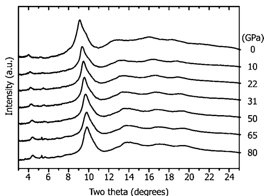
Figure 11. Stacked plot of XRD data obtained during decompression from 80 GPa. The high pressure zirconolite-II phase identified from analysis of the diffraction data at 40 GPa has fully transformed into a further polymorph with a distorted cubic structure (zirconolite-III) by around 70 GPa. These data show that this phase is recoverable to ambient conditions.
