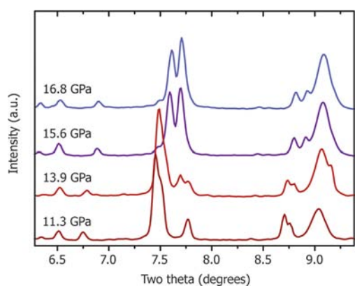
Figure 8. XRD diffraction collected at ESRF ID27 ( \lambda = 0.3738 Å) for zirconolite ( \text{CaZrTi}_2\text{O}_7 ) at high pressure in a DAC using a He as a pressure transmitting medium. A clear change in the diffraction pattern is observed between 13.9 and 15.6 GPa indicating transformation into a high-pressure phase (zirconolite-II).
