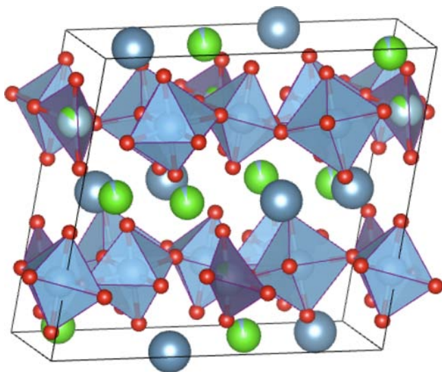
Figure 1. Structural model of the starting ambient phase of \text{CaZrTi}_2\text{O}_7 ( C2/c ). Color code: Ca atoms, large and in dark gray, Zr atoms and \text{ZrO}_7 polyhedra in green, Ti atoms and \text{TiO}_6 polyhedra in light gray, \text{Ti}(\text{Zr})\text{O}_4 tetrahedra in purple.
