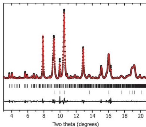
Figure 10. Le Bail refinement carried out at 40 GPa of the high pressure phase of zirconolite-II ( \text{CaZrTi}_2\text{O}_7 ). The unit cell is defined as monoclinic with a , b , and c as 9.626(4) Å, 6.672(3) Å, and 8.855(3) Å, respectively, and \beta as 102.8(2)^\circ . There are two indistinguishable space groups that fulfill the reflection conditions ( 0k0: k = 2n ), i.e., systematic absences, P2_1 and P2_1/m . Data points and Le Bail fit are presented in black and red, respectively. The upper set of tick marks is the allowed reflection positions and the lower set the reflection positions of rhenium from the DAC gasket.
