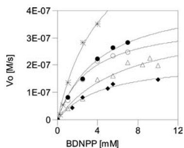
Figure 9. Michaelis–Menten plots for the hydrolysis of BDNPP catalyzed by [Co_2(CO_2EtH_2L1)(CH_3COO)_2](PF_6) (o), [Co_2(CO_2EtL2)(CH_3COO)_2](PF_6) (●), [Co_2(CH_3L2)(CH_3COO)_2](PF_6) (◆), [Co_2(NO_2L2)(CH_3COO)_2](PF_6) (Δ), and [Co_2(BrL2)(CH_3COO)_2](PF_6) (*).
