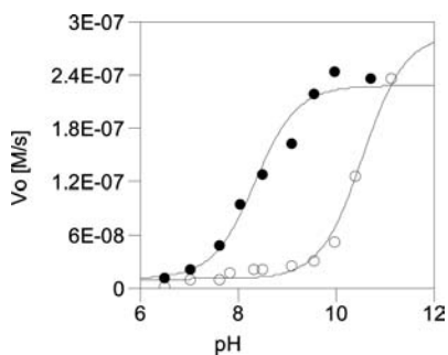
Figure 7. pH dependence profiles for [Co_2(CO_2EtH_2L1)(CH_3COO)_2](PF_6) (o) and [Co_2(CO_2EtL2)(CH_3COO)_2](PF_6) (●).
