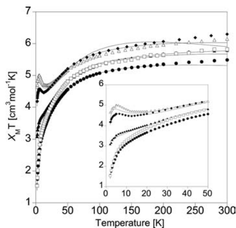
Figure 2. Plot of \chi_M T versus T for powdered samples of the complexes ( [\text{Co}_2(\text{CO}_2\text{EtH}_2\text{L1})(\text{CH}_3\text{COO})_2](\text{PF}_6) = \bullet , [\text{Co}_2(\text{CO}_2\text{EtL2})(\text{CH}_3\text{COO})_2](\text{PF}_6) = \blacktriangle , [\text{Co}_2(\text{CH}_3\text{L2})(\text{CH}_3\text{COO})_2](\text{PF}_6) = \square , [\text{Co}_2(\text{BrL2})(\text{CH}_3\text{COO})_2](\text{PF}_6) = \blacklozenge , [\text{Co}_2(\text{NO}_2\text{L2})(\text{CH}_3\text{COO})_2](\text{PF}_6) = \triangle ). The solid lines represent the best fit obtained with MagSaki software. Calculated parameters are shown in Table 3. Inset: low temperature data for the complexes.
