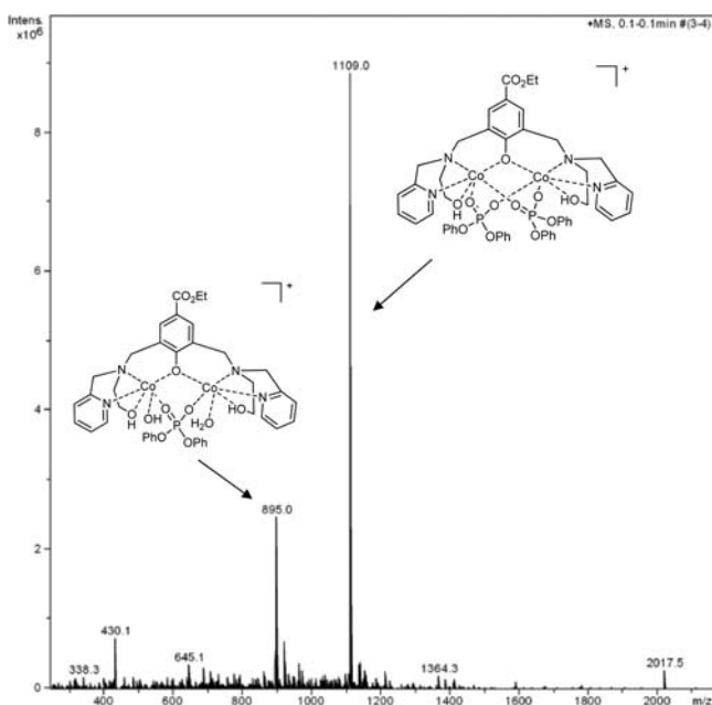
Figure 5. Mass spectrum of [\text{Co}_2(\text{CO}_2\text{EtH}_2\text{L1})(\text{CH}_3\text{COO})_2]^+ in the presence of 25 equiv of diphenyl phosphate measured in MeCN. [\text{Co}_2(\text{CO}_2\text{EtH}_2\text{L1})(\text{CH}_3\text{COO})_2]^+ was added to a solution of diphenylphosphate in MeCN (0.01 mM final concentration of complex and 0.25 mM DPP) 10 min prior to spectra recording.
