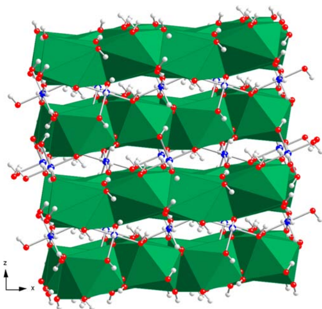
Figure 8. Three-dimensional stacking of layers in \text{Ba}_2\text{Pt}(\text{OH})_8 (5), as viewed down [010]. \text{Ba}(\text{OH})_9 polyhedra are shown in green, Pt atoms are blue spheres, O atoms are red spheres, and H atoms are gray spheres.
