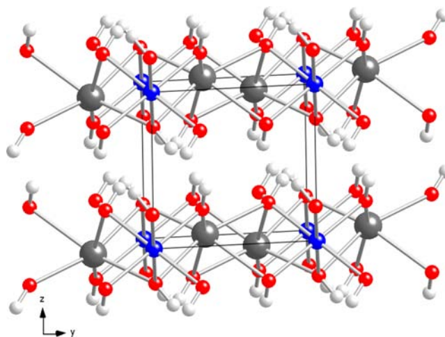
Figure 3. Crystal structure of \text{A}_2\text{Pt}(\text{OH})_6 ( A = \text{Li} (2), \text{Na} (3)), as viewed down [100]. A atoms are shown as black spheres, Pt atoms are blue spheres, O atoms are red spheres, and H atoms are gray spheres.
