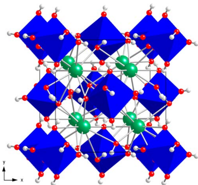
Figure 7. Crystal structure of \text{Ba}_2\text{Pt}(\text{OH})_8 (5), as viewed down [001]. Ba atoms are shown as green spheres, \text{Pt}(\text{OH})_6 octahedra are blue, O atoms are red spheres, and H atoms are gray spheres.
