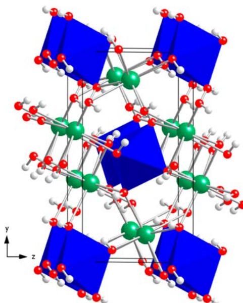
Figure 5. Crystal structure of Sr_2Pt(OH)_8 (4), as viewed down [100] . Sr atoms are shown as green spheres, Pt(OH)_6 octahedra are blue, O atoms are red spheres, and H atoms are gray spheres.
