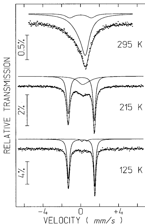
Figure 2. Mössbauer spectra of 1 at 125, 215, and 295 K.
