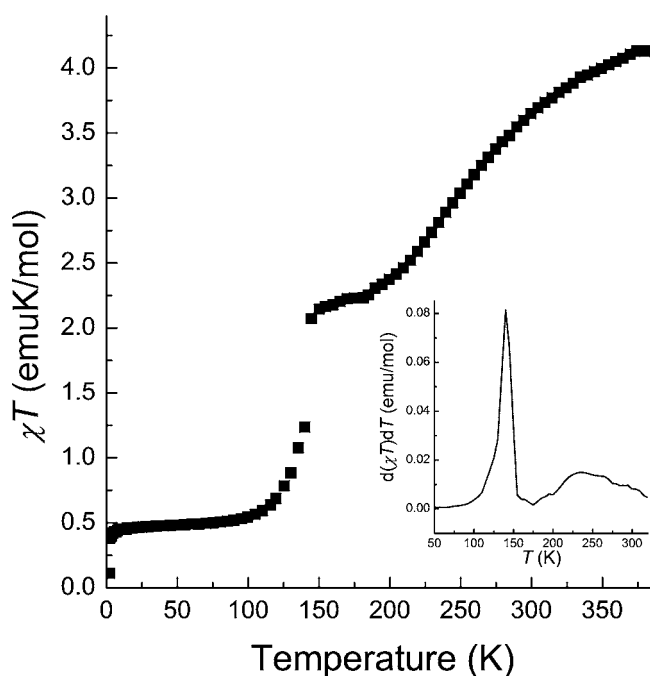
Figure 1. \chi T temperature dependence for 1 . The inset shows the first derivative of \chi T in the 50–380 K range.
