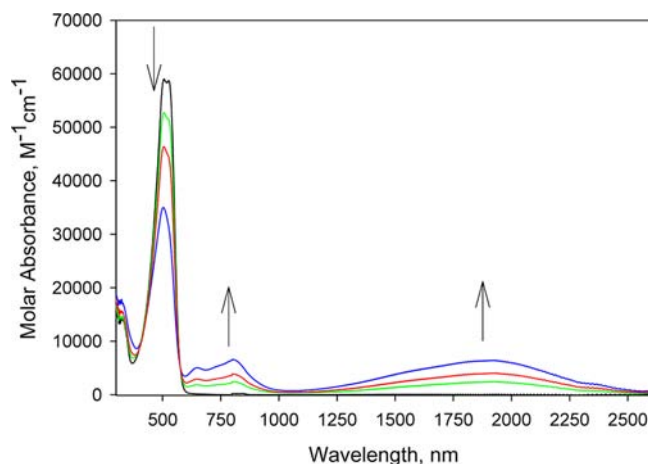
Figure 8. Spectroelectrochemistry of [\{\text{Ru}(\text{Tp})(\text{dppe})\}_2(\mu\text{-adpc})] in DMF, 0.1 M TBAH, under increasing oxidation potentials (0.0–0.93 V vs AgCl/Ag).
