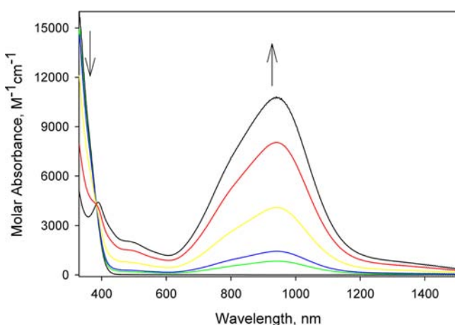
Figure 3. Spectroelectrochemistry of [\text{Ru}(\text{Tp})(\text{dppe})(\text{Cl}_5\text{pcyd})] in DMF, 0.1 M TBAH, under increasing oxidation potentials (0–0.6 V vs AgCl/Ag).
