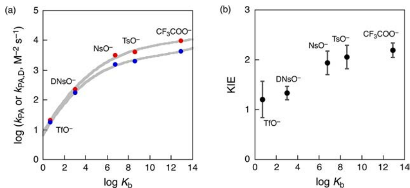
Figure 5. (a) Plots of \log k_{\text{PA}} and k_{\text{PA,D}} for reaction between [\text{Fe}^{\text{III}}(\text{OH})(\text{N4Py})]^{2+} and [\text{Ru}^{\text{III}}(\text{bpy})_3]^{3+} vs \log K_{\text{b}} performed in the presence of PA and 0.56 M \text{H}_2\text{O} (red) and \text{D}_2\text{O} (blue) in MeCN at 298 K. (b) Plots of KIE vs \log K_{\text{b}} . KIE values are determined by dividing k_{\text{PA}} by k_{\text{PA,D}} .
