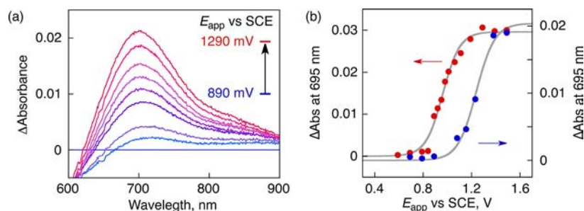
Figure 6. (a) Differential spectral changes of [\text{Fe}^{\text{III}}(\text{OH})(\text{N4Py})]^{2+} solution (0.20 mM) in the presence of \text{H}_2\text{O} (0.56 M) and \text{TsO}^- (10 mM) in MeCN at 298 K. (b) Plots of differential absorption change vs applied potential in the absence (blue) and presence of \text{TsO}^- (red) (10 mM).
