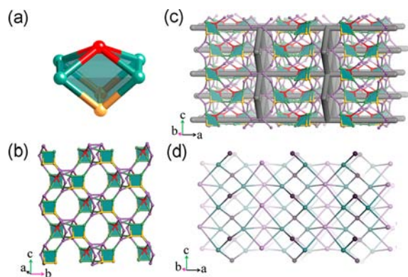
Figure 4. (a) Ge 7 cluster consisting of one GeO 6 octahedron (red), two GeO 5 trigonal bipyramids (yellow), and four GeO 4 tetrahedra (green). (b) Layer built of Ge 7 clusters and extra tetrahedral GeO 3 (OH) units (violet). (c) Framework structure with a three-dimensional channel system constructed by assembling the layers. (d) Simplified topological view of the framework, Ge 7 (green), two GeO 3 (OH) units (violet), and six GeO 3 (OH) units (violet).
