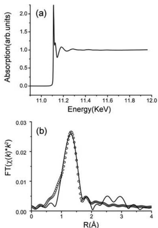
Figure 5. (a) Experimental XAFS data of GeO-JU90 plotted in E space. (b) Experimental FT-EXAFS (solid line) and best fit (open circle) in R space. Fitting was done with a k range of 2.7–13.0 Å -1 .
