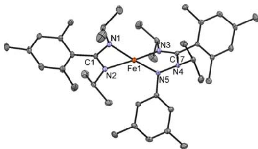
Figure 4. Molecular structure of [\text{Fe}(\text{MesC}(\text{NPr}^i)_2)(\text{NPr}^i\text{NC}_6\text{H}_3\text{-}3,5\text{-Me}_2)(\text{MesC}(\text{NPr}^i)_2)] ( 4a ) showing 30% probability ellipsoids and the partial atom numbering schemes. Selected distances (Å) and angles (deg): Fe1–N1 2.038(2), Fe1–N2 2.059(2), Fe1–N3 2.044(2), Fe1–N5 2.004(2), C1–N1 1.338(3), C1–N2 1.326(3), C17–N3 1.302(2), C17–N4 1.370(2), N4–N5 1.433(2), N1–Fe1–N2 65.5(7), N3–Fe1–N5 80.3(6), N1–Fe1–N5 125.8(7), N2–Fe1–N3 124.2(7), N1–C1–N2 112.6(2), N3–C17–N4 118.7(2), C17–N4–N5 115.3(2).
