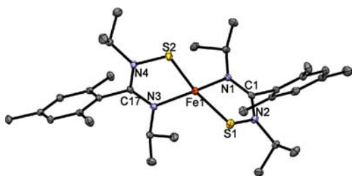
Figure 3. Molecular structure of [\text{Fe}(\text{MesC}(\text{NPr}^i)(\text{NPr}^i\text{S}))_2] ( 3 ) showing 30% probability ellipsoids and the partial atom numbering schemes. Selected distances (Å) and angles (deg): Fe1–S1 2.283(8), Fe1–S2 2.272(8), Fe1–N1 2.036(2), Fe1–N3 2.030(2), S1–N2 1.755(2), S2–N4 1.755(2), C1–N1 1.318(3), C1–N2 1.348(3), C17–N3 1.321(3), C17–N4 1.344(3), S1–Fe1–S2 127.9(3), N1–Fe1–N3 124.7(8), N1–Fe1–S1 84.8(6), N3–Fe1–S2 85.2(6), N1–Fe1–S2 119.6(6), N3–Fe1–S1 119.6(6), N1–C1–N2 119.8(2), N3–C17–N4 120.3(2).
