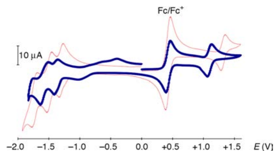
Figure 3. Cyclic voltammogram of [\text{Ru}(\text{bpy})_3](\text{PF}_6)_2 (red thin line) and complex 3e (blue bold line) in MeCN with ferrocene as internal standard ( E_{1/2}(\text{Fc}/\text{Fc}^+) = 0.41 V vs SCE).
