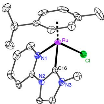
Figure 1. ORTEP representation of complex 2a (50% probability level; hydrogen atoms and noncoordinated \text{PF}_6^- anion omitted for clarity). Selected bond lengths and angles: \text{Ru1}-\text{C16} 2.009(2) Å, \text{Ru1}-\text{N1} 2.092(18) Å, \text{Ru1}-\text{Cl} 2.401(6) Å, \text{Ru}-\text{C}_{\text{centroid}} 1.710(1) Å; \text{C16}-\text{Ru1}-\text{N1} 76.42(7)^\circ .
