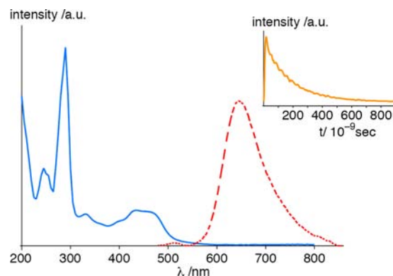
Figure 2. Absorption (blue solid line) and emission spectra (red dashed line) upon excitation at 355 nm and intensity decay (inset) for 3e in MeCN.
