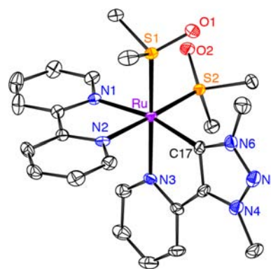
Figure 4. ORTEP representation of complex 5 (50% probability level, hydrogen atoms, and the two noncoordinated \text{PF}_6^- anions omitted for clarity). Selected bond lengths and angles: Ru1–C17 2.064(4) Å, Ru1–N3 2.149(2) Å, Ru1–N2 2.111(3) Å, Ru1–N1 2.137(3) Å, Ru1–S1 2.262(6) Å, Ru1–S2 2.2684(9) Å, C17–Ru1–N3 77.99(13)°, N1–Ru1–N2 77.50(12)°, S1–Ru1–S2 89.14(3)°.
