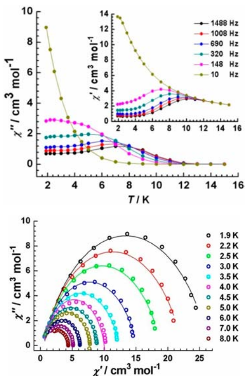
Figure 7. Temperature dependence of the in-phase ( \chi' ) and out-of-phase ( \chi'' ) ac susceptibility signals for 2 under zero dc field (up). The solid lines are a guide for the eyes; Cole–Cole plots under zero-dc field for compound 2 (bottom). The solid lines indicate the fits using a generalized Debye model.
