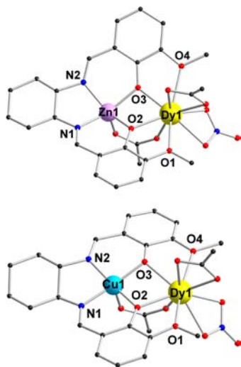
Figure 1. Molecular structures of 1 (up) and 3 (bottom). Hydrogen atoms and solvent molecules are omitted for clarity. Color scheme: yellow, Dy; purple, Zn; sky blue, Cu; red, O; blue, N; gray, C.
