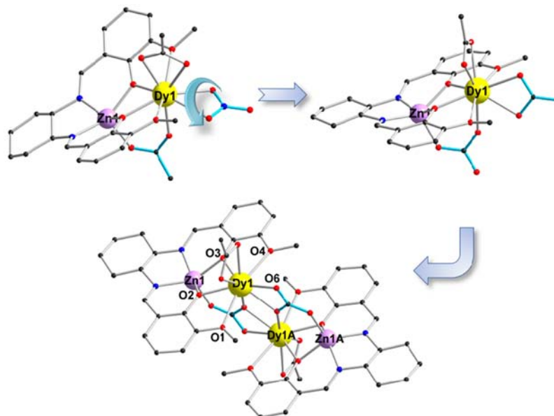
Figure 2. Crystal structure of compound 2 and its assembly from [\text{ZnDy}] building blocks (1).
