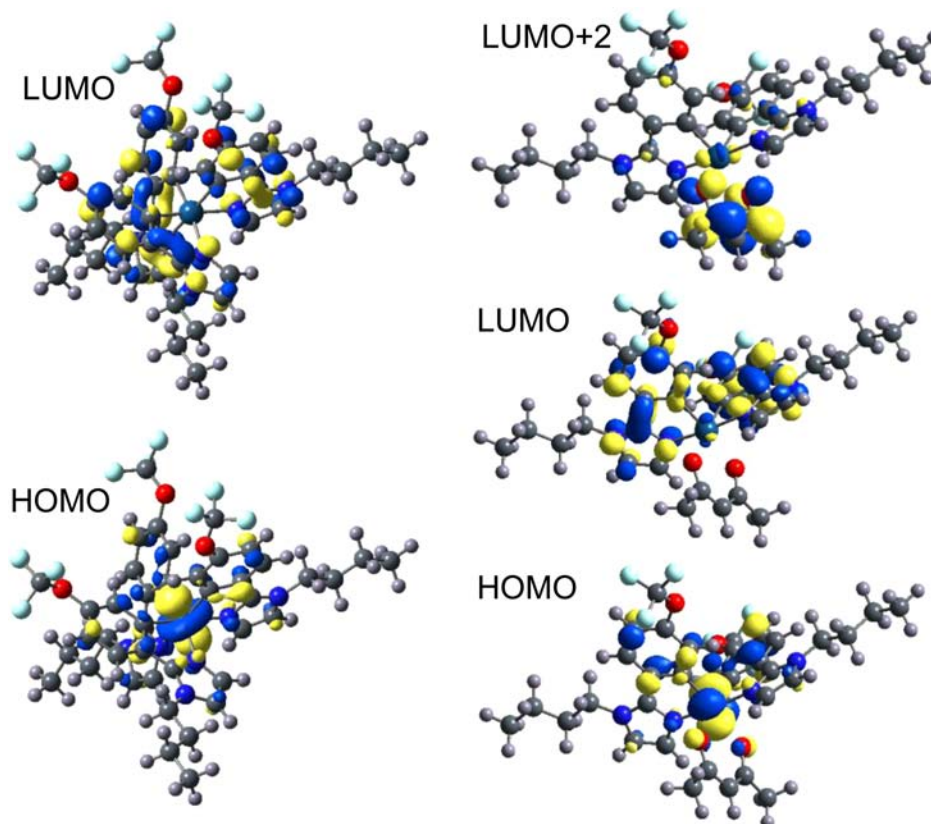
Figure 3. MOs of fac -OCF 3 (left side) and OCF 3 acac (right side).
