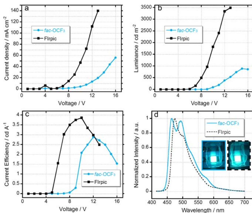
Figure 11. (a) J - V , (b) L - V , and (c) \eta - V characteristics. (d) EL spectra and photographs of the fabricated devices.
