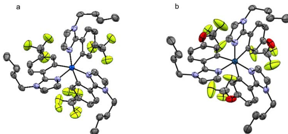
Figure 2. ORTEP diagram of (a) fac -CF 3 and (b) fac -OCF 3 (hydrogen atoms are neglected for clarity).
