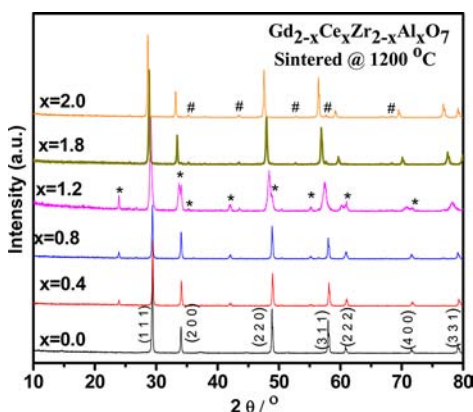
Figure 3. XRD patterns of Gd_{2-x}Ce_xZr_{2-x}Al_xO_7 sintered at 1200\text{ }^\circ\text{C} in air (*, GdAlO_3 phase; #, Al_2O_3 and unmarked peaks are due to fluorite type phase for composition see Table 1).
