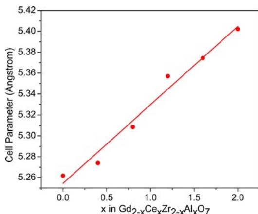
Figure 2. Cell parameter variation as function of x in Gd_{2-x}Ce_xZr_{2-x}Al_xO_7 calcined at 700\text{ }^\circ\text{C} .
