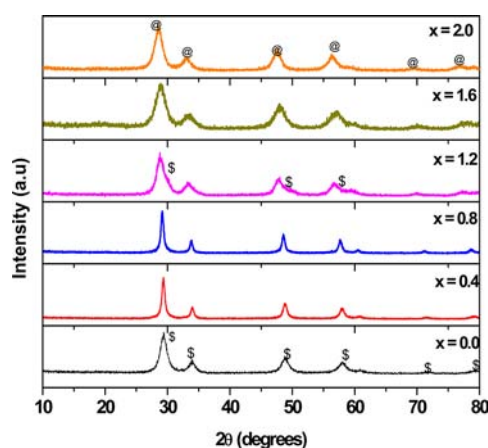
Figure 1. XRD pattern of as-prepared Gd 2-x Ce x Zr 2-x Al x O 7 compositions calcined at 700 °C ($, Gd-rich phase; @, Ce-rich phase).
