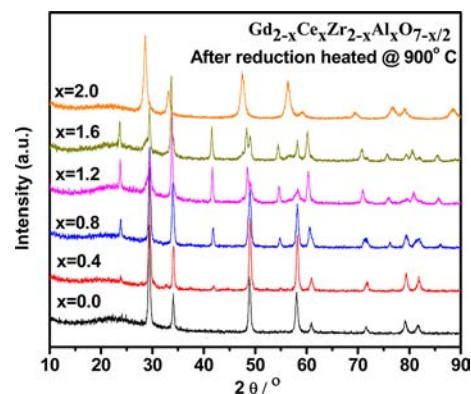
Figure 5. XRD pattern of reduced \text{Gd}_{2-x}\text{Ce}_x\text{Zr}_{2-x}\text{Al}_x\text{O}_{7-x/2} after heating at 900 °C in air.
