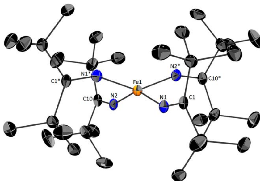
Figure 3. Solid-state molecular structure of [\text{Li}(12\text{-crown-4})_2][\text{Fe}(\text{N}=\text{C}^t\text{Bu}_2)_4] ( 5 ) with 40% probability ellipsoids. [\text{Li}(12\text{-crown-4})_2]^+ and hydrogen atoms are excluded for clarity. Atoms with an asterisk are generated by symmetry. Selected bond lengths (Å) and angles (deg): \text{Fe1-N1} = 1.859(3) , \text{Fe1-N2} = 1.858(4) ; \text{N1-Fe1-N2} = 145.02(14) , \text{N1-Fe1-N1}^* = 94.0(2) , \text{Fe1-N1-C1} = 154.9(3) , \text{Fe1-N2-C10} = 156.6(3) .
