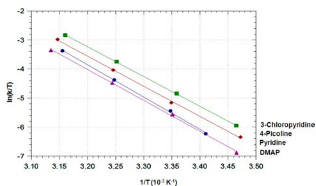
Figure 4. Eyring plots [ \ln(k/T) vs 1/T ] for the reaction of fac -[Re(Sal- mTol )(CO) 3 (HOCH 3 )] with various pyridine type ligands in methanol.
