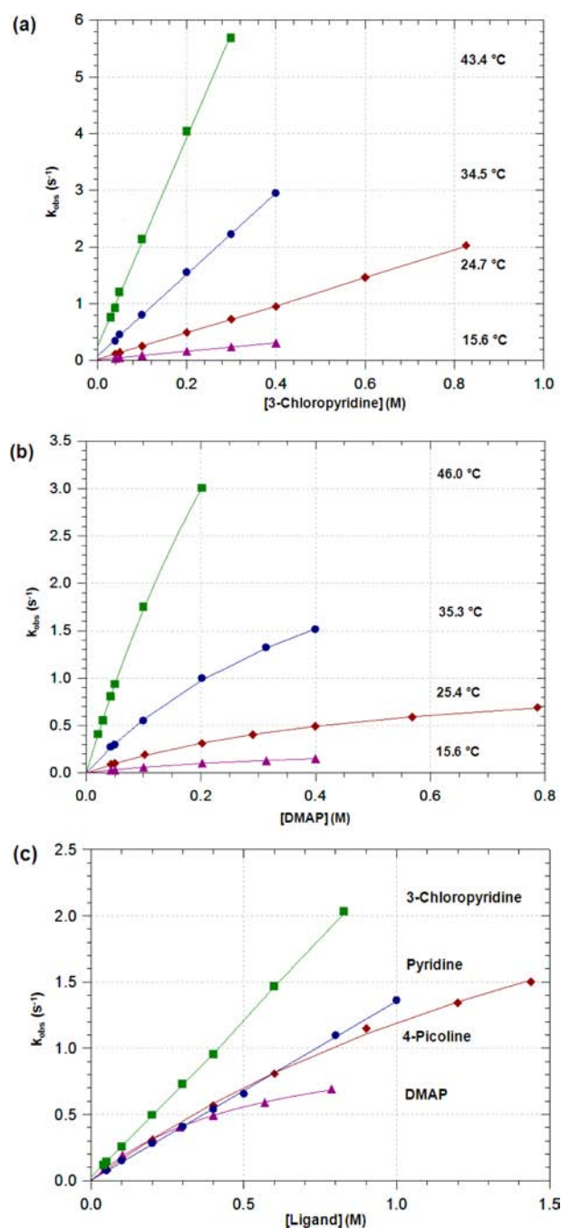
Figure 3. Plot of k_{\text{obs}} vs entering ligand for the reaction of (a) fac -[Re(Sal- mTol )(CO) 3 (HOCH 3 )] and 3-chloropyridine at various temperatures in methanol, yielding linear plots, [Re complex] = 4.38 \times 10^{-4} M, ( \lambda = 436 nm); (b) fac -[Re(Sal- mTol )(CO) 3 (HOCH 3 )] and DMAP at various temperatures in methanol yield limiting plots, [Re complex] = 5.19 \times 10^{-4} M, ( \lambda = 440 nm); (c) fac -[Re(Sal- mTol )(CO) 3 (HOCH 3 )] and various entering ligands at 25 °C in methanol.
