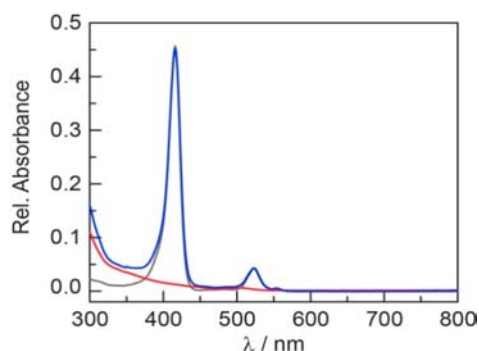
Figure 6. Comparison of the absorption spectra of 1 (gray lines), QD (red lines) and QD1 (blue lines) in toluene. The spectrum of QD1 represents a composite of the two constituent spectra.
