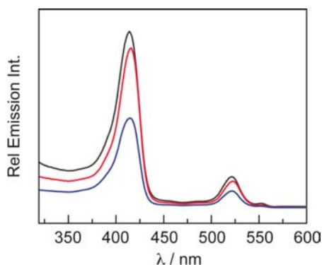
Figure 8. Excitation spectra ( \lambda_{em} = 685 nm) of concentration-matched toluene solutions of QD1 (black lines), QD2 (red lines), and QD3 (blue lines).
