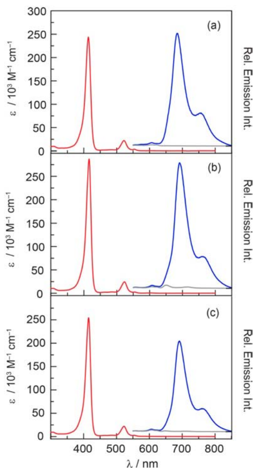
Figure 4. Comparison of the steady state absorption (red lines) and emission spectra ( \lambda_{\text{exc}} = 525 nm) of (a) 1 , (b) 2 , and (c) 3 in the presence of air ( \sim 160 Torr O 2 ) (gray lines) and under vacuum (blue lines) in toluene.
