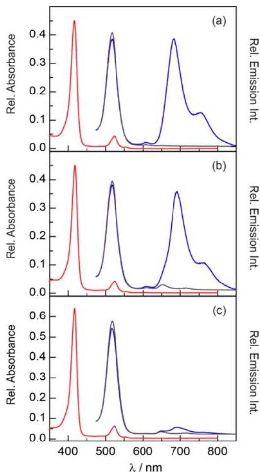
Figure 7. Comparison of the steady state absorption (red lines) and emission spectra ( \lambda_{\text{exc}} = 525 nm) of (a) QD1 , (b) QD2 , and (c) QD3 in the presence of air ( \sim 160 Torr \text{O}_2 ) (gray lines) and under vacuum (blue lines) in toluene.
