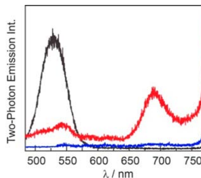
Figure 9. Two-photon emission spectra ( \lambda_{exc} = 800 nm) of concentration-matched toluene solutions of QD (black lines) and freeze–pump–thawed solutions of 1 (blue lines) and QD1 (red lines). 1 does not emit under two-photon excitation, and emission is only observable in the presence of QD .
