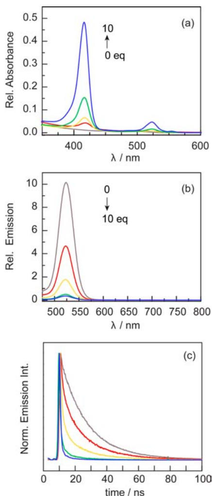
Figure 5. Spectral changes associated with titration of a toluene solution of QD (gray lines) with 1 (red lines), 2 (yellow lines), 5 (green lines), and 10 (blue lines) equiv of 1 . Similar data for 2 and 3 are shown in Supporting Information, Figures S3 and S4. (a) The intensity of the Soret and Q-band absorption profiles increases. (b) The QD emission ( \lambda_{\text{exc}} = 450 nm) intensity is quenched, and (c) the decay profiles of the QD emission ( \lambda_{\text{exc}} = 450 nm) decrease with increasing equiv of 1 .
