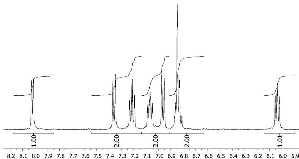
Figure 1. ^1\text{H} NMR spectrum of the dodecanuclear complex 1 (400 MHz, \text{CD}_2\text{Cl}_2 ). Resonances assignable to six of the eight protons associated with each [2\text{-phenylpyridine}(-\text{H})] ligand are fully resolved, with the remaining two resonances overlapping between 6.8 and 6.9 ppm.
