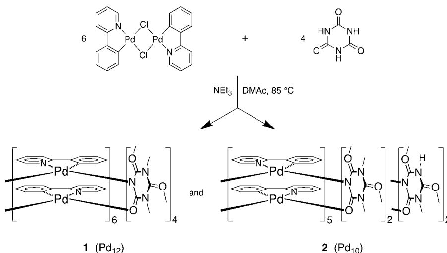
Scheme 1. Formation of the Dodecapalladium and Decapalladium Cage-Complexes 1 and 2 , Respectively, from Reaction of [\text{Pd}\{2\text{-phenylpyridine}(-\text{H})\}\text{-}\mu\text{-Cl}]_2 with Cyanuric Acid
