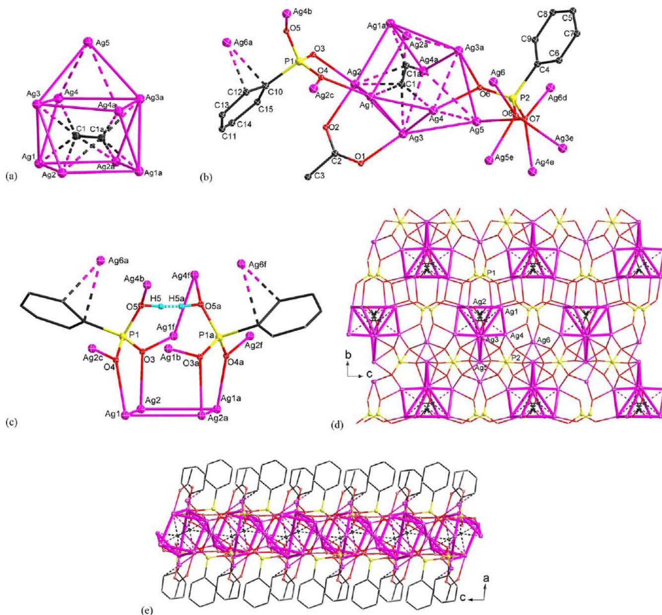
Figure 1. (a) The C_2@Ag_9 building block of 1 in the shape of a distorted monocapped square antiprism. Ag...Ag distances longer than 3.4 Å (twice the van der Waals radius of silver) are represented by broken lines. Selected bond lengths and distances [Å]: C1≡C1a 1.248(2), Ag...Ag 2.773(8)–3.378(9). (b) Asymmetric unit in the crystal structure of 1 , showing the C_2@Ag_9 cage, the coordination modes of the trifluoroacetate and phosphonate groups, and the \eta^2 -coordination of the phenyl group to Ag6. The F and H atoms are omitted for clarity. (c) The coordination mode of the P1 group, showing the [C_6H_5PO_3 \cdots H \cdots O_3PC_6H_5]^{3-} assembly. (d) Layer structure of 1 viewed along the a axis, in which the C_2@Ag_9 cages are linked by phosphonate groups. The phenyl moieties, H, and F atoms are omitted for clarity. (e) Layer structure of 1 viewed along the b axis. The H and F atoms are omitted for clarity. Symmetry codes: (a) 1 - x, y, 1.5 - z ; (b) 1 - x, 1 - y, 2 - z ; (c) x, 1 - y, 0.5 + z ; (d) x, -y, -0.5 + z ; (e) 1 - x, -y, 2 - z ; (f) x, 1 - y, -0.5 + z ; (g) 1 - x, 1 - y, 1 - z .
