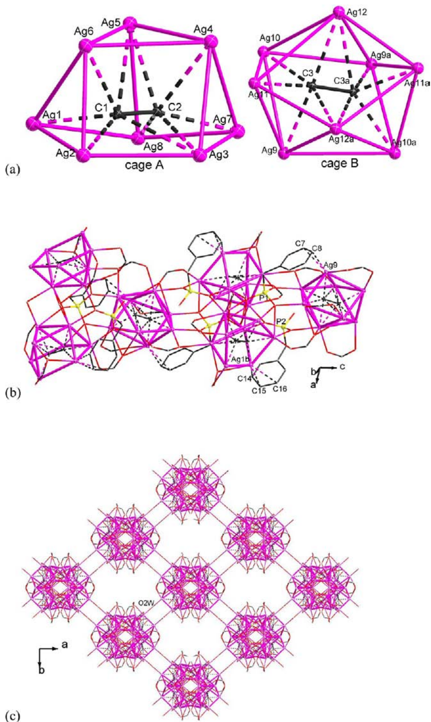
Figure 7. (a) Two types of irregular polyhedra existing in the compound 7 . Selected bond lengths and distances [ \text{\AA} ]: \text{C1}\equiv\text{C2} 1.24(1), \text{C3}\equiv\text{C3a} 1.24(2), \text{Ag}\cdots\text{Ag} 2.794(1)–3.354(1). (b) Perspective view of coordination silver chain constructed of silver cages in the form of \text{A}_2\text{BA}_2\text{B}\cdots . The unimportant atoms are omitted for clarity. (c) Three-dimensional coordination architecture of 7 generated from the cross-linkage of silver chains by coordination with aqua ligands O2W. The unimportant atoms are omitted for clarity. Symmetry codes: (a) 1-x, y, 0.5-z ; (b) 1-x, 1-y, -z ; (c) 0.5-x, 1.5-y, -z .
