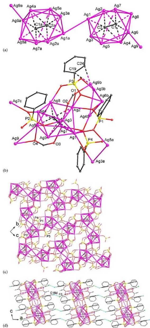
Figure 3. (a) Basic building unit in 3 consisting of a \text{C}_2@Ag_8 cage with an extended arm; two such units are connected by vertex-to-vertex linkage across an inversion center. Ag...Ag distances longer than 3.40 Å are represented by broken lines. Selected bond lengths and distances [Å]: \text{C}\equiv\text{C} 1.23(1), Ag...Ag 2.831(1)–3.365(1), Ag9b–C24 2.592(1), Ag9b–C19, 2.754(1). (b) Asymmetric unit in the crystal structure of 3 , showing the single silver cage and the coordination modes of the phosphonate and trifluoroacetate ligands. The H atoms are omitted for clarity. (c) View of the layer structure of 3 parallel to the bc plane, in which the silver aggregates are linked by phosphonate groups. The phenyl moieties of the phosphonate groups, H, and F atoms are omitted for clarity. (d) Three-dimensional supramolecular framework of 3 generated from the linkage of layers by weak C–H...F hydrogen bonds involving trifluoroacetate and phosphonate groups, which are represented by broken lines. Symmetry codes: (a) 0.5 - x, 0.5 - y, -z ; (b) 0.5 - x, 0.5 + y, 0.5 - z ; (c) 0.5 - x, -0.5 + y, 0.5 - z ; (d) -0.5 + x, 0.5 + y, z .
