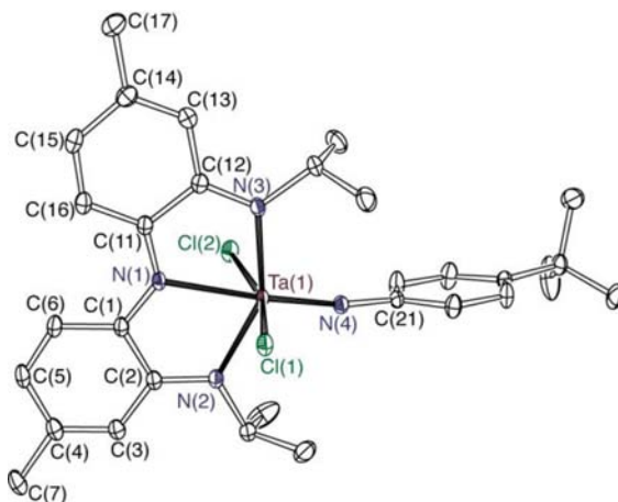
Figure 7. ORTEP diagram for \text{Me}_i\text{Pr}(\text{NNN}^{\text{q}})\text{TaCl}_2(=\text{N-p-C}_6\text{H}_4\text{tBu}) ( 7d ). Thermal ellipsoids are drawn at 50% probability. Hydrogen atoms and cocrystallized solvent molecules have been omitted for clarity.
