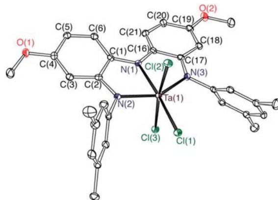
Figure 5. ORTEP diagram for \text{OMe,DMP}(\text{NNN}^{\text{sq}})\text{TaCl}_3 ( 6f ). Thermal ellipsoids are drawn at 50% probability. Hydrogen atoms and cocrystallized solvent molecules have been omitted for clarity.
