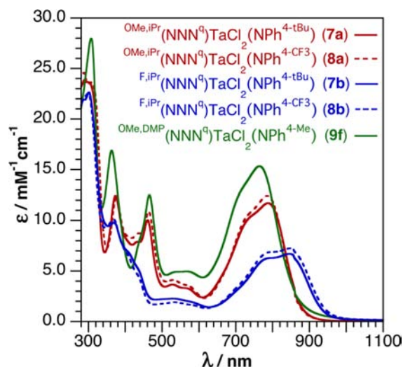
Figure 6. UV–vis–NIR spectra of \text{OMe}_i\text{Pr}(\text{NNN}^{\text{q}})\text{TaCl}_2(\text{NPh}^{4\text{-tBu}}) ( 7a ), \text{OMe}_i\text{Pr}(\text{NNN}^{\text{q}})\text{TaCl}_2(\text{NPh}^{4\text{-CF}_3}) ( 8a ), \text{F}_i\text{Pr}(\text{NNN}^{\text{q}})\text{TaCl}_2(\text{NPh}^{4\text{-tBu}}) ( 7b ), \text{F}_i\text{Pr}(\text{NNN}^{\text{q}})\text{TaCl}_2(\text{NPh}^{4\text{-CF}_3}) ( 8b ), and \text{OMe,DMP}(\text{NNN}^{\text{q}})\text{TaCl}_2(\text{NPh}^{4\text{-Me}}) ( 9f ) collected at 298 K in THF.
