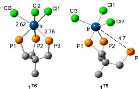
Figure 4. Optimized DFT (M06/LANL2DZ) 5- and 6-coordinate triplets \mathbf{1}^{\text{T5}} and \mathbf{1}^{\text{T6}} (hydrogen atoms and phenyl rings omitted).
