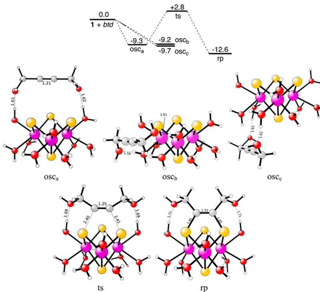
Figure 10. Computed free energy profile (kcal/mol) for the reaction between btd and 1 , with the structures (Å) of outer-sphere complexes ( osc ), transition state ( ts ), and reaction product ( rp ). Color code: green = Cl; purple = Mo; yellow = S; gray = C; red = O; white = H.
