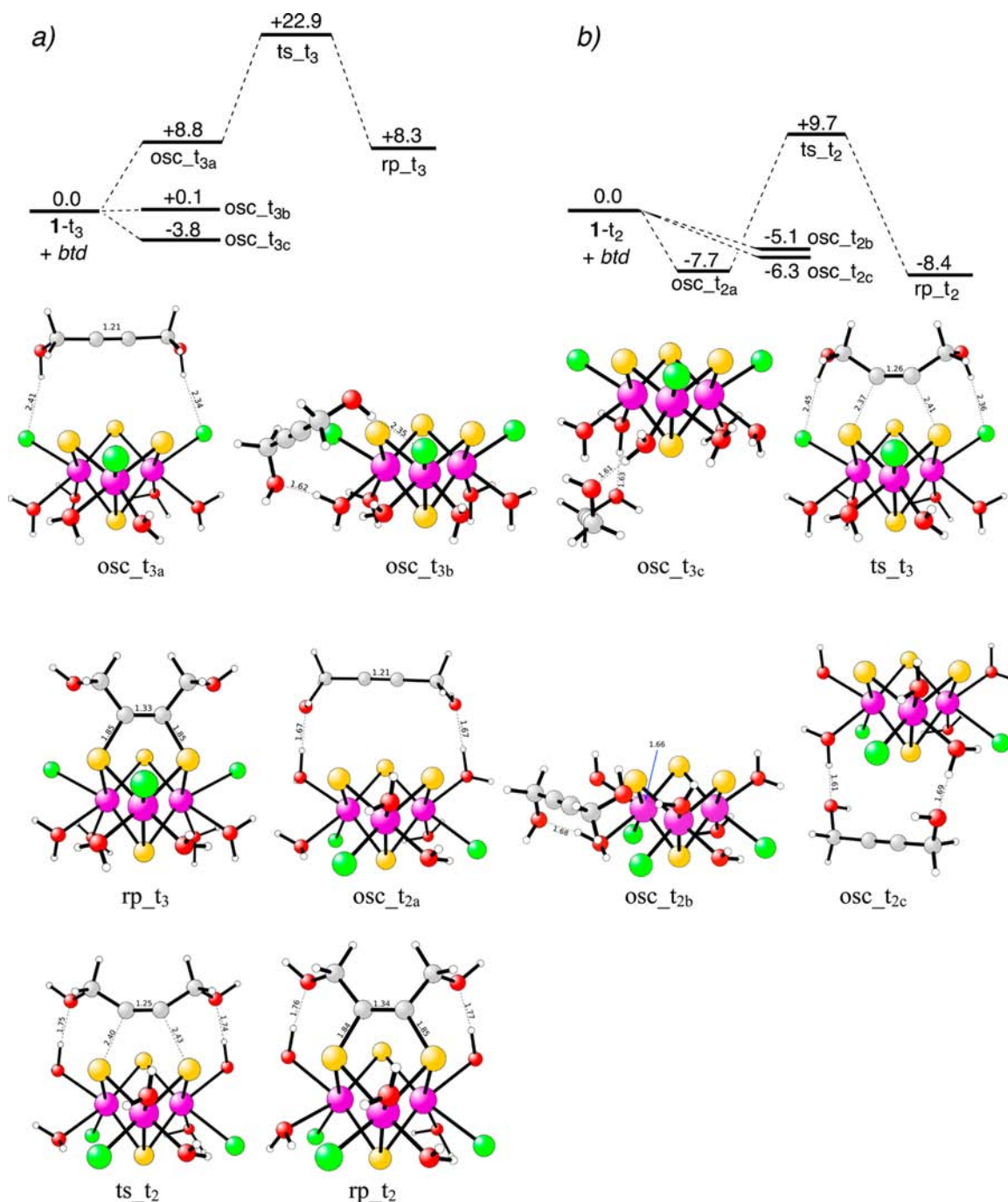
Figure 11. Computed free energy profile (kcal/mol) for the reaction between btd and [\text{Mo}_3\text{S}_4\text{Cl}_3(\text{H}_2\text{O})_6]^+ , with Cl ligands trans to \mu_3 -S (1- t_3 , a), and trans to \mu_2 -S (1- t_2 , b), with the structures (Å) of outer-sphere complexes (osc), transition states (ts), and products (rp). Note that in the case of 1- t_3 , higher-energy osc featuring OH...Cl interactions are not shown for simplicity (included in the Supporting Information). Color code: green = Cl; purple = Mo; yellow = S; gray = C; red = O; white = H.
