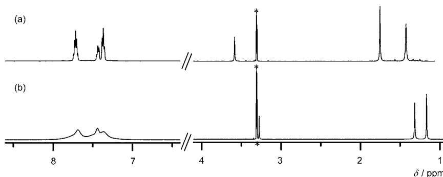
Figure 1. 1 H NMR spectra of (a) [H 2 1] and (b) [H2] in methanol- d 4 at ambient temperature. Asterisks (*) denote signals from the solvent.
