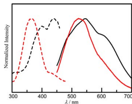
Figure 6. Emission (solid line) and excitation (dashed line) spectra of [3] (black) and [4]\text{Cl} (red) in the solid state.
