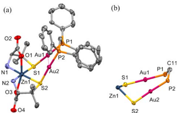
Figure 3. ORTEP drawings of (a) the entire trinuclear complex molecule and (b) the 8-membered metalloring structure in [3]. One of the two independent complex molecules is selected. H atoms are omitted for clarity.
