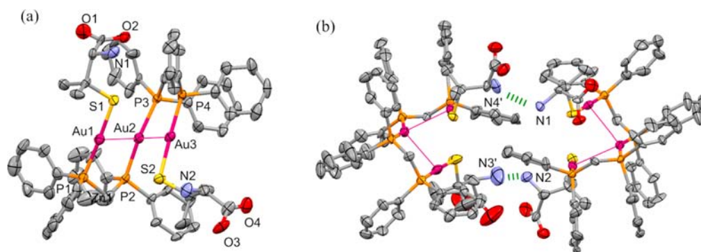
Figure 2. ORTEP drawings of (a) one of two crystallographically independent trigold(I) complex molecules of [H2] and (b) its dimeric structure. H atoms are omitted for clarity. Green dashed lines indicate the hydrogen-bonding interactions. Symmetry code ('): x, 1 + y, -1 + z .
