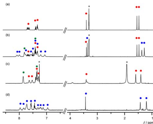
Figure 5. 1 H NMR spectra of (a) [3] and (b) [4]Cl in methanol- d 4 , (c) [4]Cl in chloroform- d , and (d) [4]Cl in D 2 O. Red, blue, and green circles indicate the signals from [3], [4] + , and [Au 2 (dppm) 2 ]Cl 2 , respectively. Asterisks (*) denote signals from the solvents.
