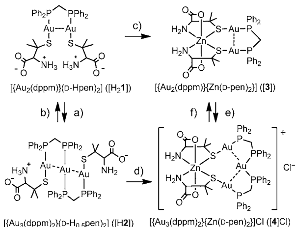
Scheme 1. Synthetic Routes to [H 2 1], [H2], [3], and [4]Cl +
