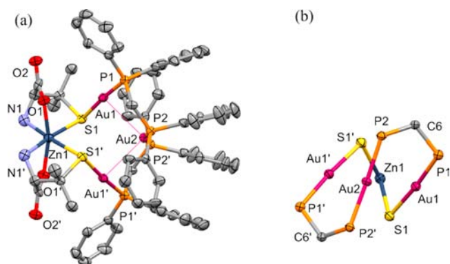
Figure 4. ORTEP drawings of (a) the entire tetranuclear complex cation and (b) the 12-membered metalloring structure in [4]Cl. H atoms are omitted for clarity.
