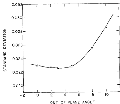
Figure 5.—Standard deviations for the converged sets of parameters for a sequence of out-of-plane angles.
