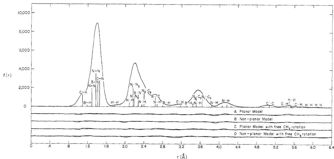
Figure 4.—The refined radial distribution curve for (\text{CH}_3)_2\text{N}_4\text{BH} and the difference curves between the experimental and theoretical functions for different models.
