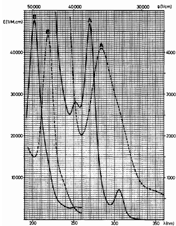
Fig. 3. Solution absorption spectra of [\text{Pt}(\text{DEPE})_2](\text{ClO}_4)_2 (—) and [\text{Pt}(\text{PEt}_3)_4](\text{ClO}_4)_2 (- - -).
