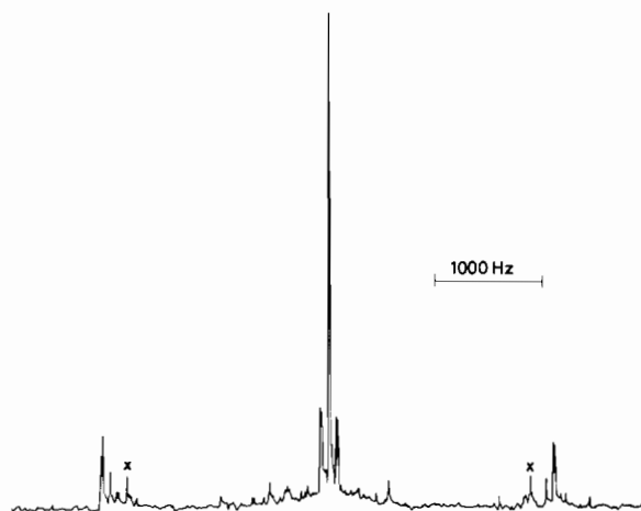
Fig. 1. ^{31}\text{P}\{^1\text{H}\} NMR spectrum of [\text{Pt}_2\text{Cl}_2(\mu\text{-Ph}_2\text{PCH}_2\text{SMe})_2] . Peaks marked x are ^{195}\text{Pt} satellites of the decomposition product (see text).
