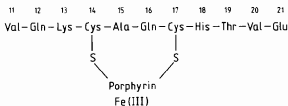
Fig. 1. The amino acid sequence of HUP^{III} . The numbering of the residues refers to native cytochrome c (from ref. 11).
