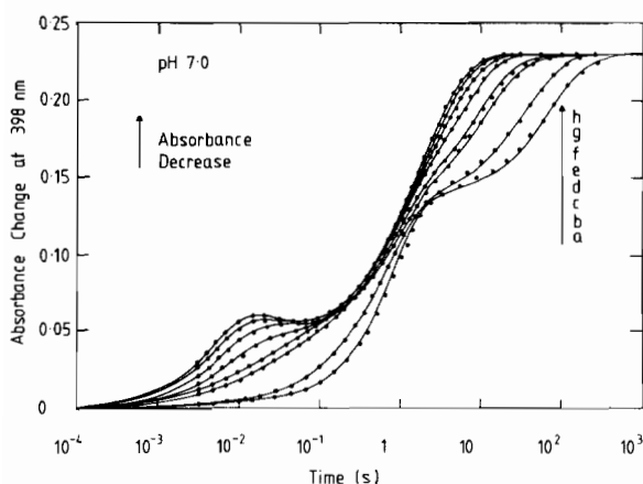
Fig. 2. Observed and computed kinetics of the reaction of HUP III with H 2 O 2 at pH 7.0 monitored at 398 nm. Symbols: ●, observed time courses; —, best fit computed time curves for the scheme at pH 7.0 shown in Table II. Experimental conditions: 1.63 μM (final concentration in the mixing chamber) HUP III in 0.1 M sodium phosphate buffer pH 7.0 at 22 °C (syringe 1) was reacted with H 2 O 2 dissolved in the same buffer (syringe 2). The final concentrations of H 2 O 2 in the reaction chamber were: (a) 1.29 mM, (b) 2.58 mM, (c) 7.79 mM, (d) 10.3 mM, (e) 16.5 mM, (f) 22.8 mM, (g) 28.8 mM, and (h) 33.1 mM. Path length 1.7 cm.
