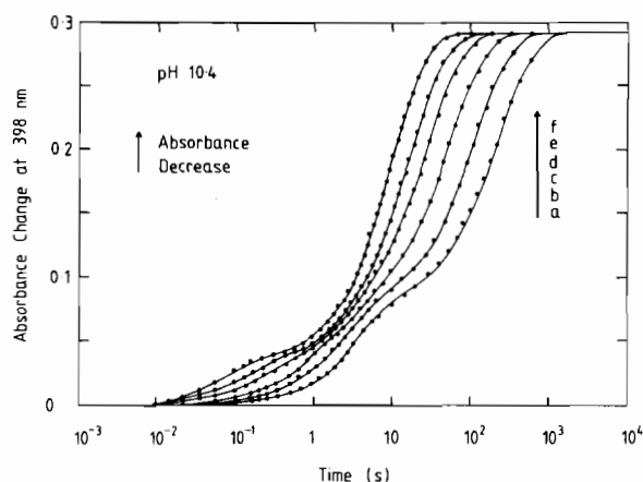
Fig. 3. Observed and computed kinetics of the reaction of HUP III with H 2 O 2 at pH 10.4 monitored at 398 nm. Symbols: ●, observed time course; —, best fit computed time courses for the scheme at pH 10.4 shown in Table II. Experimental conditions: 1.63 μM (final concentration in the mixing chamber) HUP III in 0.1 M sodium borate buffer pH 10.4 at 22 °C (syringe 1) was reacted with H 2 O 2 dissolved in the same buffer (syringe 2). The final concentrations of H 2 O 2 in the mixing chamber were: (a) 2.79 mM, (b) 5.58 mM, (c) 11.5 mM, (d) 22.3 mM, (e) 35.9 mM and (f) 71.8 mM. Path length 1.7 cm.
