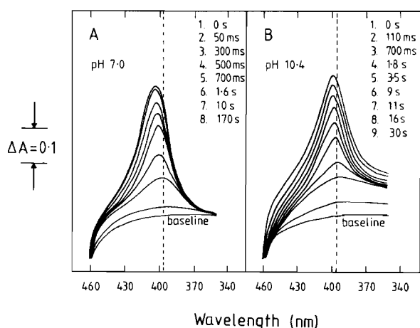
Fig. 5. Time resolved spectra in the Soret region obtained during the reactions of HUP III with H 2 O 2 at pH 7.0 (A) and 10.4 (B) by rapid wavelength scanning stopped flow optical spectroscopy. Experimental conditions: HUP III in (A) 0.1 M sodium phosphate buffer pH 7.0 and (B) 0.1 M sodium borate buffer pH 10.4 (syringe 1) was reacted with H 2 O 2 dissolved in the corresponding buffers (syringe 2) at 22 °C. The final concentration of HUP III in the mixing chamber was 3.8 μM. The final concentrations of H 2 O 2 in the mixing chamber were: 1 mM (A) and 50 mM (B). Path length 1.0 cm.
