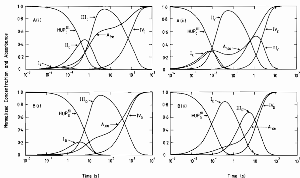
Fig. 4. Computed time courses of the concentrations of the intermediate species and absorbance changes at 398 nm in the reactions of \text{HUP}^{\text{III}} at pH 7.0 (A), and 10.4 (B) for the schemes shown in Table II. Initial conditions: 2 \mu\text{M} \text{HUP}^{\text{III}} , (i) 1 \text{ mM} and (ii) 50 \text{ mM} \text{H}_2\text{O}_2 . The values of the rate constants and difference extinction coefficients ( \text{HUP}^{\text{III}} minus intermediate species) at each pH are given in Table III.
