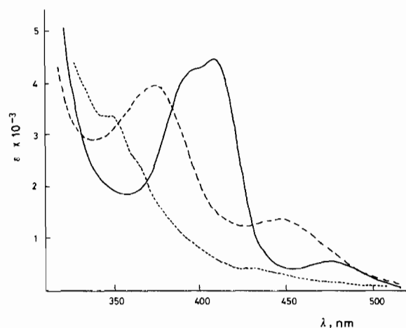
Fig. 1. Electronic spectra in MeOH of RuCl 4 (RCN) 2 - [—]; after 2 days RuCl 3 (RCN) 2 MeOH [---]; after 4 days the species RuCl 2 + [· · · · ·].
