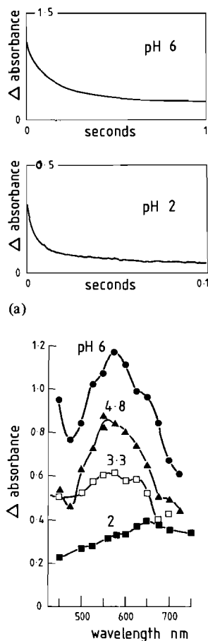
Fig. 1. (a) Stopped-flow traces of the reaction between anaerobic aqueous solutions of ascorbic acid and iron(III) chloride. Upper: the ferric chloride and ascorbic acid concentrations were 1.25 \times 10^{-2} \text{ M} and 0.1 \text{ M} respectively. The monitoring wavelength was 560 nm. Lower: the ferric chloride and ascorbic acid concentrations were 2.5 \times 10^{-3} \text{ M} and 2.5 \times 10^{-2} respectively. The monitoring wavelength was 560 nm. All reactant concentrations given are those after mixing. T = 20^\circ \text{C} . (b) Kinetic difference spectra for the reaction between anaerobic aqueous solutions of ascorbic acid and iron(III) chloride at different pH values. Conditions: Ferric chloride concentration 1.25 \times 10^{-3} \text{ M} ; ascorbate concentration 1.25 \times 10^{-2} \text{ M} ; pH 6.0. Ferric chloride concentration 1.25 \times 10^{-3} \text{ M} ; ascorbic acid concentrations 1.2 \times 10^{-3} \text{ M} ; pH 4.8. Ferric chloride concentration 1.25 \times 10^{-3} \text{ M} ; ascorbic acid concentration 1.2 \times 10^{-3} \text{ M} ; pH 3.3. Ferric chloride concentration 2.5 \times 10^{-3} \text{ M} ; ascorbic acid concentration 2 \times 10^{-1} \text{ M} ; pH 2.0. All reactant concentrations given are those before mixing.
