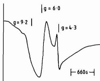
Fig. 3. EPR spectrum of a FeCl 3 /GSH solution (red) in a 1:10 ratio at pH 9.0. [FeCl 3 ] = 1 mM. The sample was frozen immediately after equilibrating with oxygen. The conditions of EPR spectroscopy were: microwave power, 2mW; microwave frequency, 9.43 GHz; modulation amplitude, 2 mT; temperature, 15 K.
