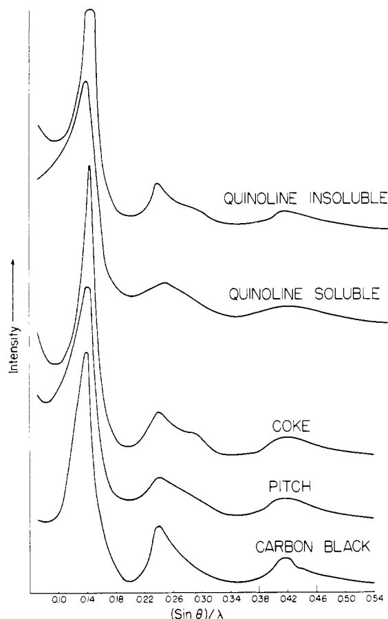
Figure 1. Comparison of the wide-angle x-ray diffraction patterns of an electrode binder pitch, its 575^\circ\text{C} . coke, quinoline-soluble and insoluble fractions of a pitch, and a typical carbon black
