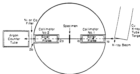
Figure 4. Schematic diagram of small-angle scattering apparatus
