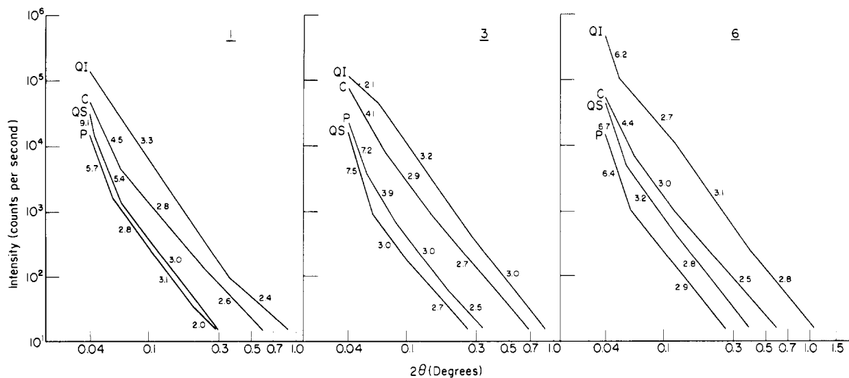
Figure 5. Plots of \log_{10} I vs. \log_{10} 2\theta for three electrode binder pitches, P , their 575°C cokes C , quinoline-insoluble fractions, Q. I. , and quinoline-soluble fraction, Q. S. Numbers on curves indicate magnitudes of the negative slopes
