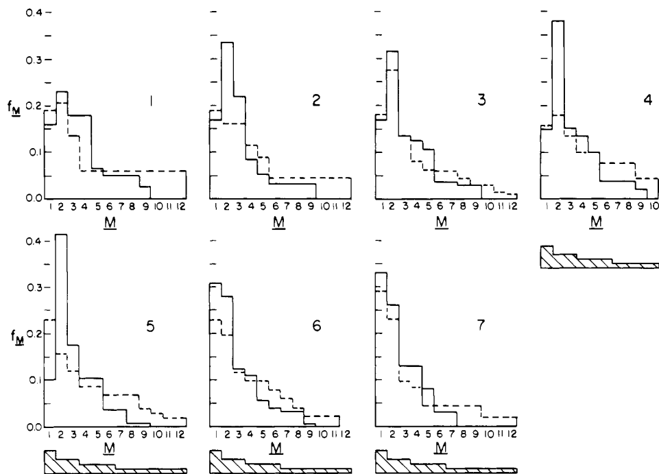
Figure 2. Histograms comparing the M distributions in six pitches (Nos. 1 to 6), a beta resin (No. 7), and their respective 575° C. cokes —Uncoked - - -Coked. Estimated precision of f_M 's indicated by hatched histograms
