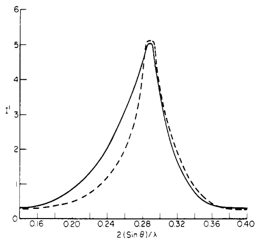
Figure 3. Comparative (002) profiles of pitch No. 3 (solid line) and its 575° C. coke (broken line)
