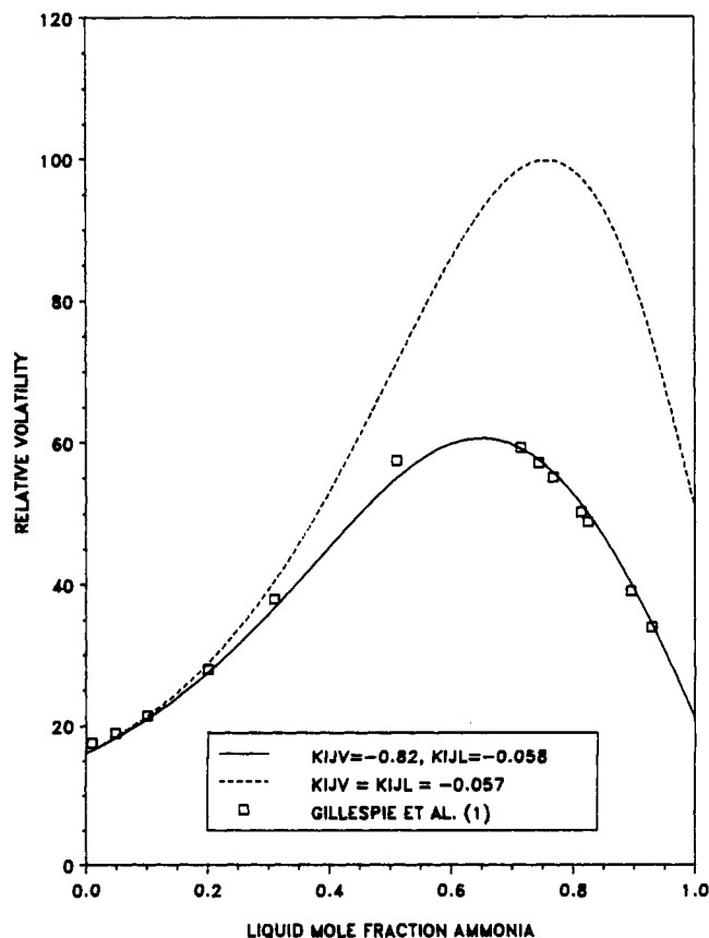
Figure 7. Relative volatility at 80 °C. Points are the data of Gillespie et al. (1), solid line is calculated with Table III parameters, and the dashed line is for K_{ij}^v = K_{ij}^l .
