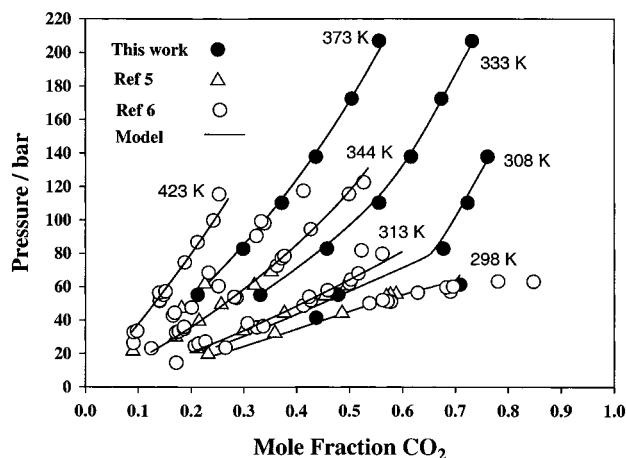
Figure 3. Comparison of high-pressure propylene carbonate-CO 2 VLE.
