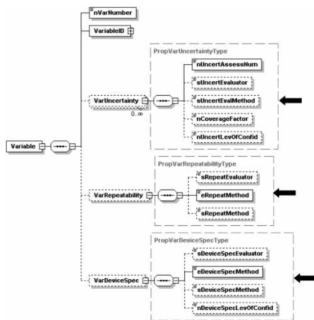
Figure 9. Structure of the Variable element in the “ ReactionData ” block. The arrows indicate new elements described in the text.
