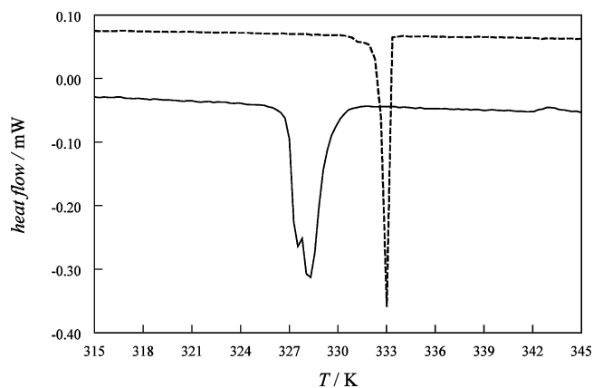
Figure 2. Crystallization of tristearin, starting at 334 K (dashed line) and 329 K (solid line) and at during the cooling of the melt with a rate of -0.1 \text{K}\cdot\text{min}^{-1} .
