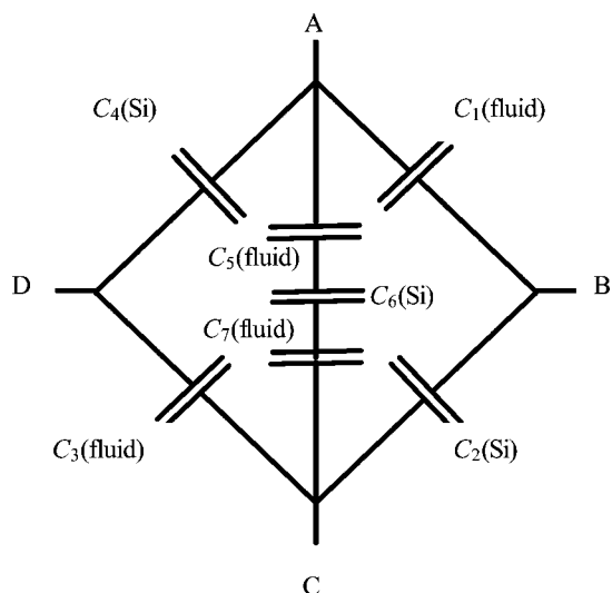
Figure 4. Schematic representation of the Wheatstone bridge configuration of the four capacitances C_n with n = 1, 2, 3, and 4 labeled A and B in Figure 3 along with connections A through D and additional contributions arising from the separation of the two fluid exposed capacitors.
