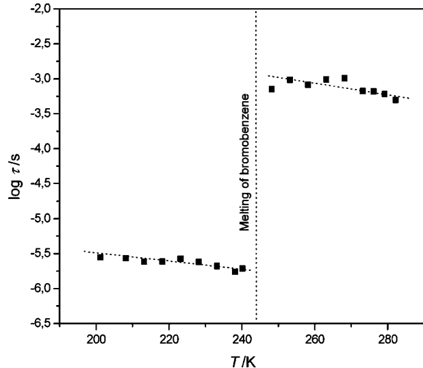
Figure 5. Dielectric relaxation time \tau vs T for \text{C}_6\text{H}_5\text{Br} .
