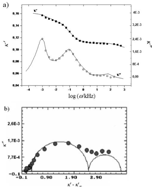
Figure 10. (a) Spectrum plot for C_6H_5Br in MWNTs of 4.0 nm diameter at 274 K; (b) representation of the spectrum plots in the form of a Cole–Cole diagram.
