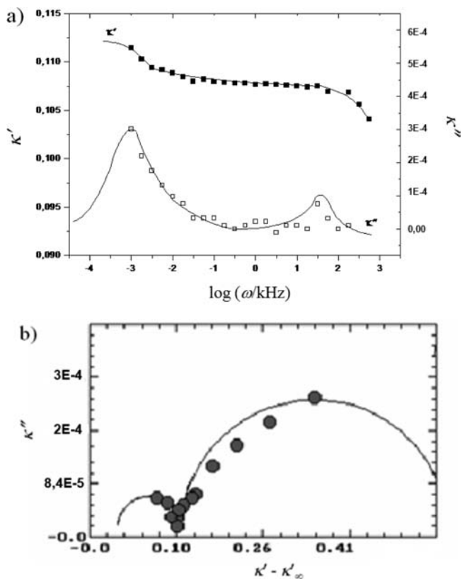
Figure 9. (a) Spectrum plot for C_6H_5Br in MWNTs of 4.0 nm diameter at 261 K; (b) representation of the spectrum plots in the form of a Cole–Cole diagram.
