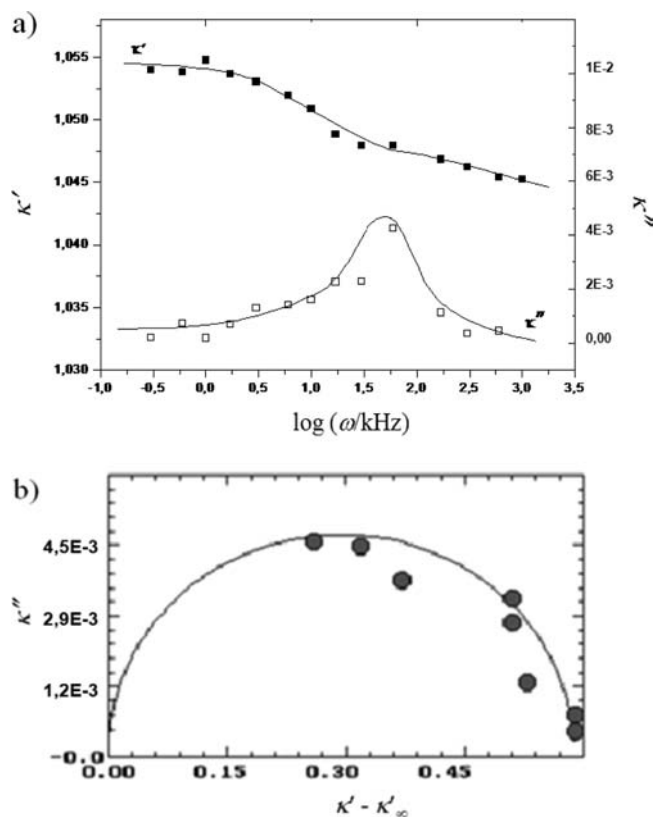
Figure 3. (a) Spectrum plot for C_6H_5Br at 209 K (the solid state); (b) representation of the spectrum plots in the form of a Cole–Cole diagram for C_6H_5Br at 209 K.
