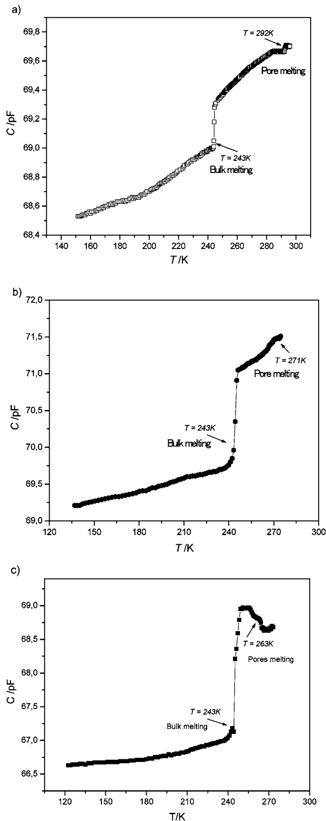
Figure 6. Electric capacity C vs temperature T for \text{C}_6\text{H}_5\text{Br} confined in MWNT: (a) 2.4 nm; (b) 4.0 nm; (c) 10 nm.
