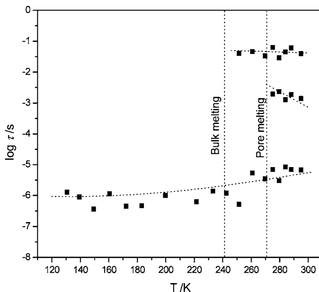
Figure 11. Dielectric relaxation time \tau vs T for C_6H_5Br in MWNTs of diameter 4.0 nm.
