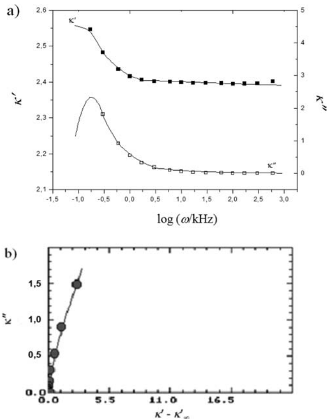
Figure 4. (a) Spectrum plot for \text{C}_6\text{H}_5\text{Br} at 267 K (the liquid state); (b) representation of the spectrum plots in the form of a Cole–Cole diagram for \text{C}_6\text{H}_5\text{Br} at 267 K.
