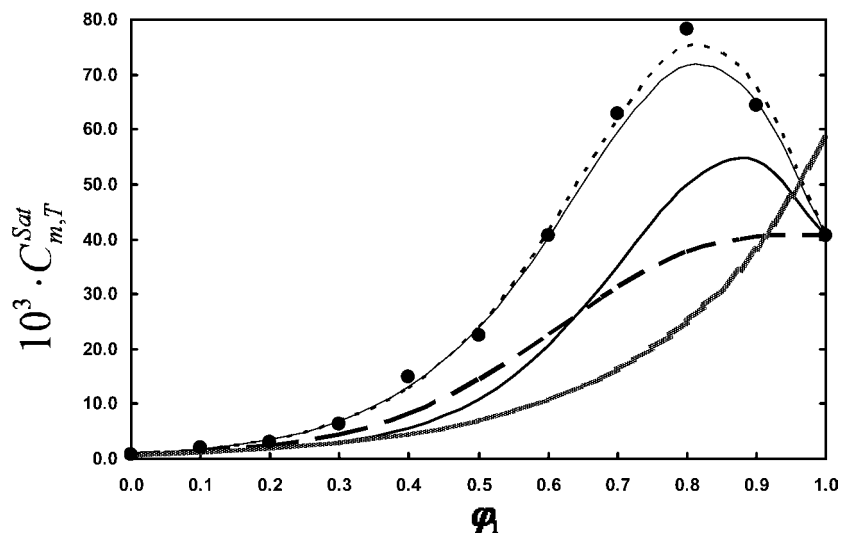
Figure 2. mol·L -1 solubility of hydrocortisone ( C_{m,T}^{\text{Sat}} ) at various volume fractions of ethanol ( \varphi_1 ) in binary solvent mixtures; ●, experimental; and the predicted solubilities using: short-dashed line, eq 1; solid line, eq 2; bold solid line, eq 3; long-dashed line, eq 4; gray patterned line, eq 5.
