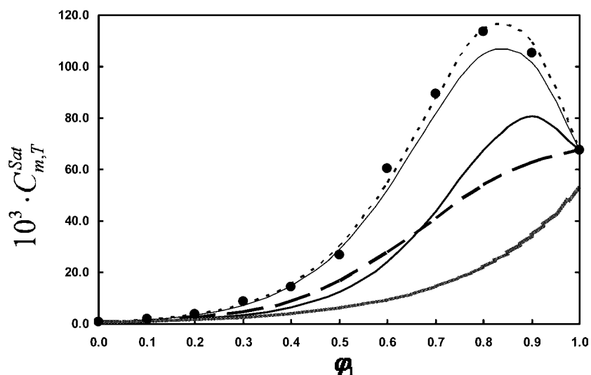
Figure 3. mol·L -1 solubility of prednisolone ( C_{m,T}^{\text{Sat}} ) at various volume fractions of ethanol ( \varphi_1 ) in binary solvent mixtures; ●, experimental; and the predicted solubilities using: short-dashed line, eq 1; solid line, eq 2; bold solid line, eq 3; long-dashed line, eq 4; gray patterned line, eq 5.
