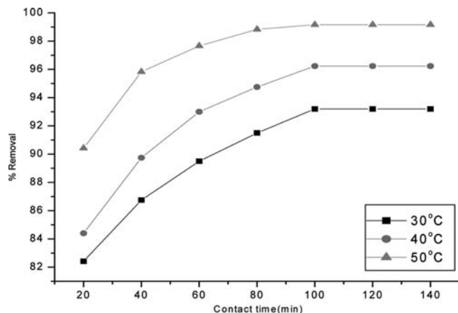
Figure 7. Effect of temperature on the percent removal of methylene blue on RHAC.
