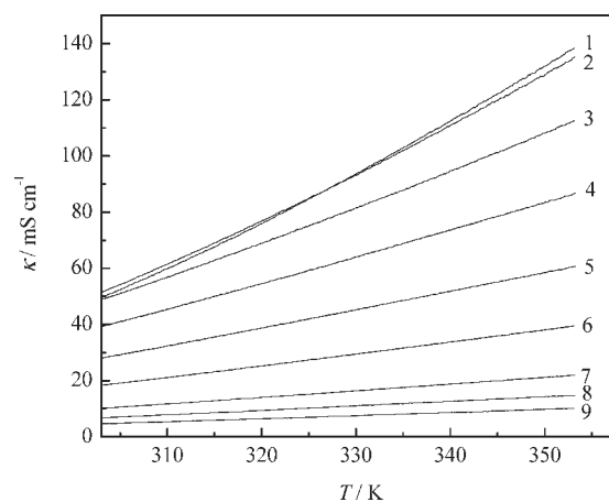
Figure 3. Electrical conductivity of ammonium nitrate + formamide mixtures vs temperature at different HCONH 2 /NH 4 NO 3 mole ratio R : 1, 1.5; 2, 2.0; 3, 5.0; 4, 10; 5, 20; 6, 40; 7, 100; 8, 200; 9, 500.
