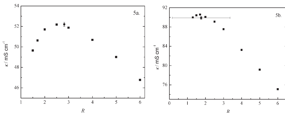
Figure 5. Comparison of the experimental obtained and calculated \kappa_{\max} value at \mu molality of ammonium nitrate (molality is recalculated and expressed as mole ratio R ) at 303.15 K (a) and 328.15 K (b): ■, experimental values; ●, calculated values.
