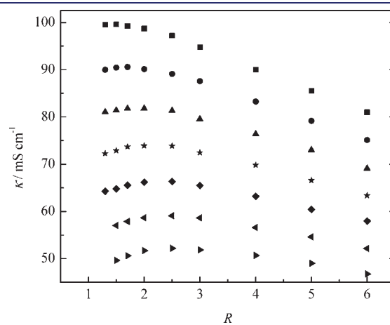
Figure 4. Electrical conductivity vs HCONH 2 /NH 4 NO 3 mole ratio R at different temperatures: right pointing triangle, 303.15 K; left pointing triangle, 313.15 K; \blacklozenge , 318.15 K; \star , 323.15 K; \bullet , 328.15 K; \blacksquare , 333.15 K.
