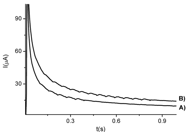
Figure 3. One-step potential chronoamperometric experiments for 6b in the presence 0.1M TBABF 4 in CH 3 CN. The initial potential was the open potential circuit value E_{\text{ocp}} . The potential step values ( E_1 ) were (a) 0.3 V/Fc-Fc + and (b) 0.8 V/Fc-Fc + .
