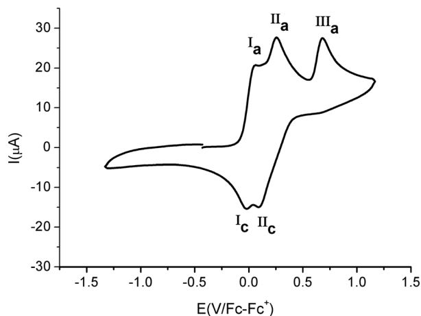
Figure 4. Cyclic voltammograms for a solution 1.0 \times 10^{-3} mol \text{dm}^{-3} of compound 5a+6a in the presence of 0.1 M TBABF 4 in acetonitrile. Working electrode platinum, scan rate 0.10 V s -1 .
