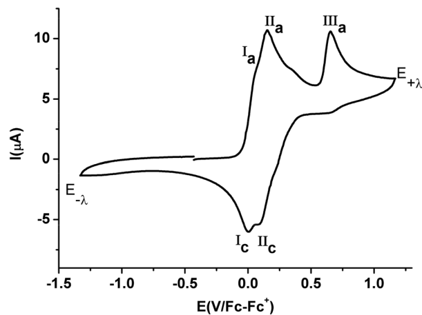
Figure 2. Cyclic voltammograms for a solution 1.0 \times 10^{-3} mol \text{dm}^{-3} of compound 6b in the presence of 0.1M TBABF 4 in acetonitrile. Working electrode platinum, scan rate 0.1 V s -1 .
