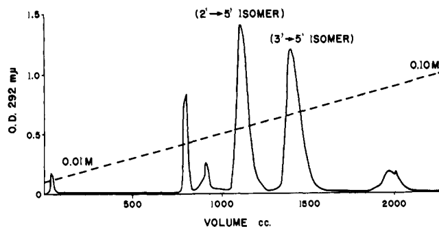
Figure 1.—Resolution of 5-methyluridylyl-(3'→5')-5-methyluridine: column, Dowex-1 × 2 (formate) 200–400 mesh, size 1.5 × 40 cm. The mixture of isomers (100 mg.) was placed on the column and the column was developed with a linear gradient of sodium formate buffer (pH 4.5) from 0.01 → 0.1 M. Ratio of the amount of the (2'→5') isomer to that of the (3'→5') isomer is 45:55.
