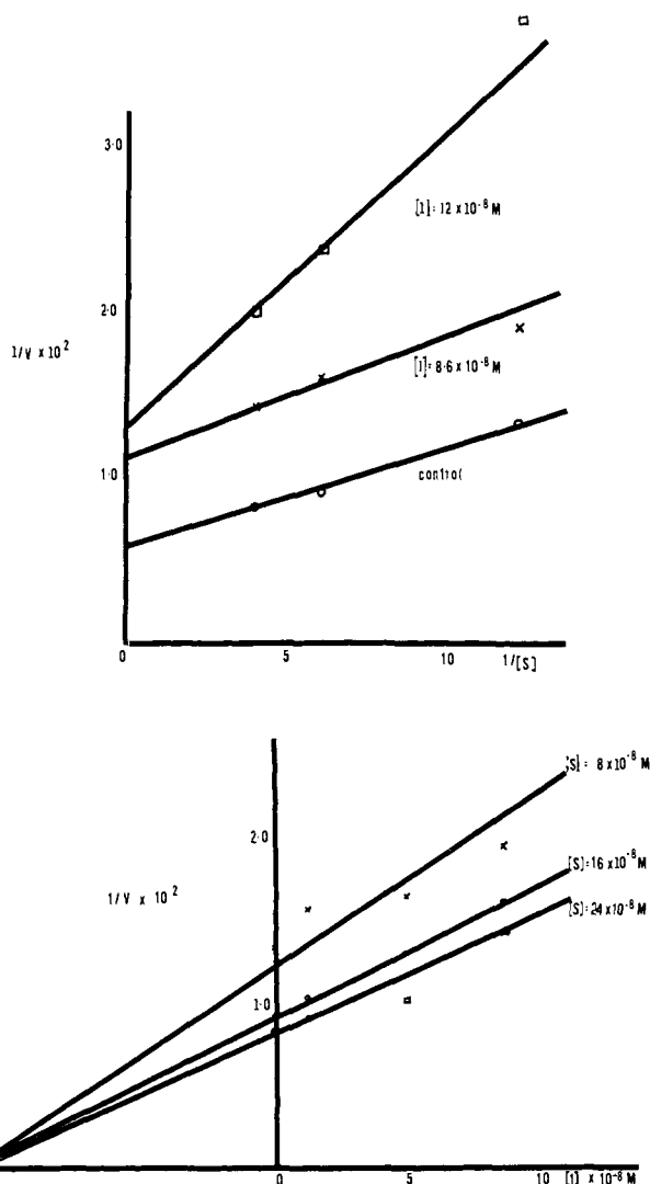
Figure 1.—Lineweaver–Burk (top) and Dixon (bottom) plots showing noncompetitive inhibition of MAO in vitro by 22 .
