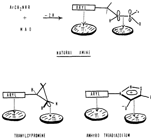
Figure 5.—Spatial relationships between natural amine substrates for MAO and the inhibitors tranlylcypromine and anhydrothiadiazolium hydroxides.
