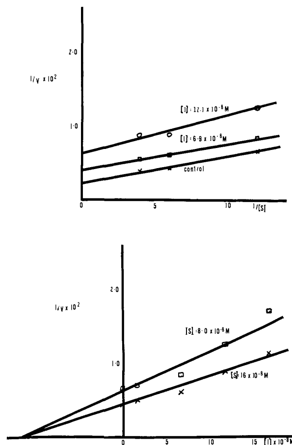
Figure 3.—Lineweaver-Burk (top) and Dixon (bottom) plots showing noncompetitive inhibition of MAO in vitro by 35 .
