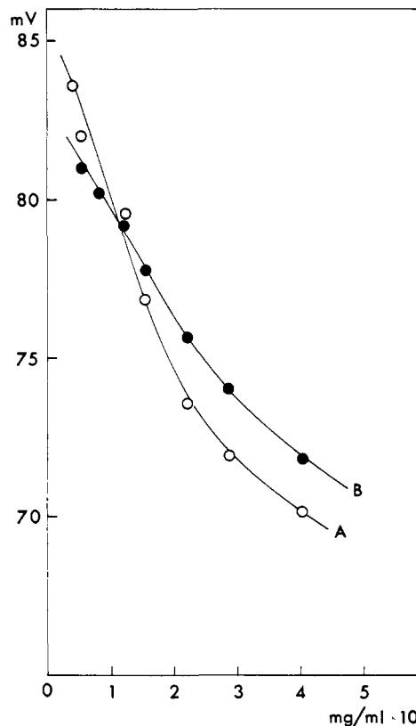
Figure 1.—Electromotive force recorded in solutions of N -( \beta -aminoethyl)polyglycine in 1 \times 10^{-4} M KCl ( \overline{DP} = 19 in plot A; \overline{DP} = 6 in plot B) vs. the polypeptide concentration.
